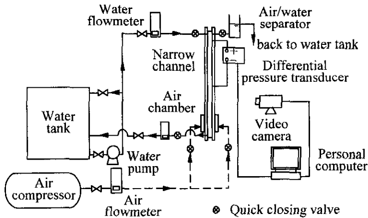
Fig. 1 Schematic of the experimental apparatus.
