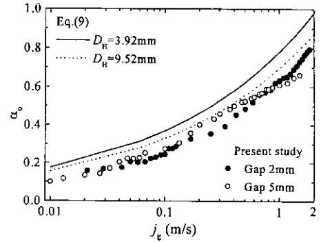
Fig. 4 Average void fraction in narrow rectangular channels with zero liquid flow.
