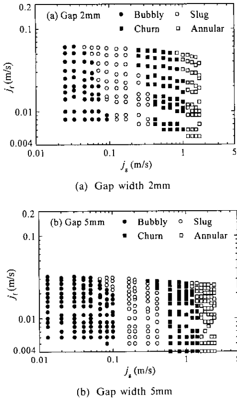
Fig. 3 Counter-current flow regimes for narrow rectangular channels.
