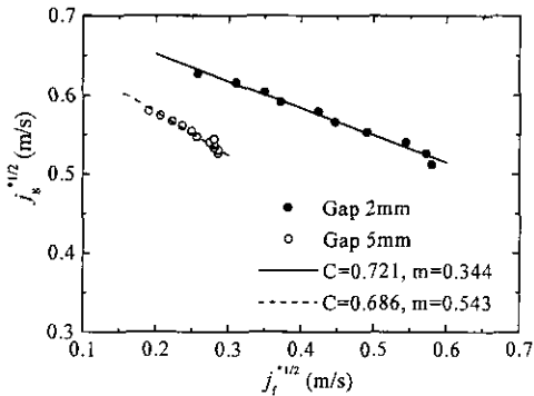
(b) Flooding curves
