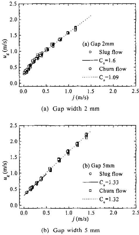
Fig. 5 Drift-flux correlation of the void fraction.
