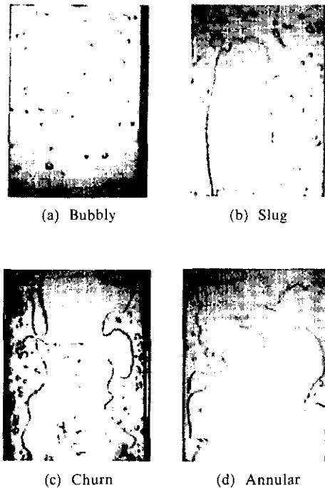
Fig. 2 Sample images of two-phase flow regimes in narrow rectangular channels.
