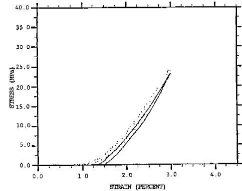
Fig. 7 Stress-strain plot for the 300 th cycle in test A-2 with 5%/sec strain rate (— : Predicted data, ···· : Measured data)
