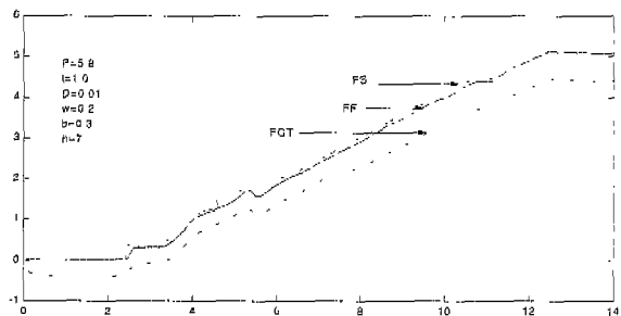
Fig. 22. Fuel loop feedback control by the NN-Tuning 2-DOF PID controller ( P=2.2 , I=0.2 , D=0.01 , w=0.2 , b=0.3 , h=7 ).
