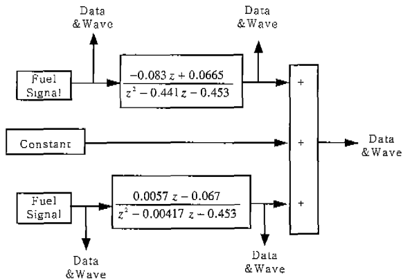
Fig. 5. The structure of transfer function in the Gun-san gas turbine.
