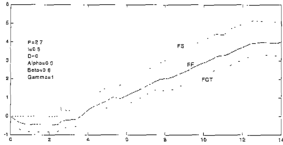
Fig. 15. Fuel loop feedback control by the conventional 2-DOF PID controller ( P=2.7 , I=0.5 , D=0.0 , \alpha=0.9 , \beta=0.6 , \gamma=1.0 )
