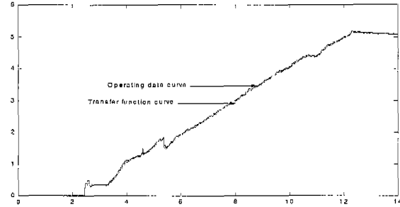
Fig. 6. Operating data curve and transfer function curve.
