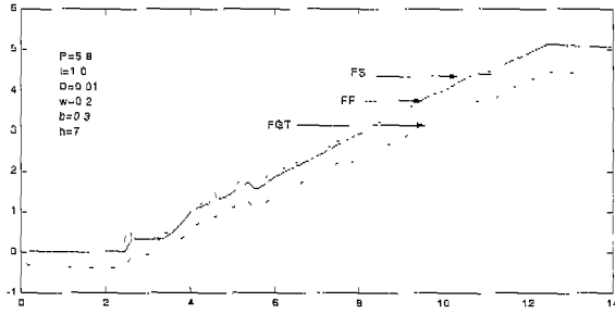
Fig. 23. Fuel loop feedback control by the NN-Tuning 2-DOF PID controller ( P=2.2 , I=0.2 , D=0.01 , w=0.2 , b=0.3 , h=7 ).
