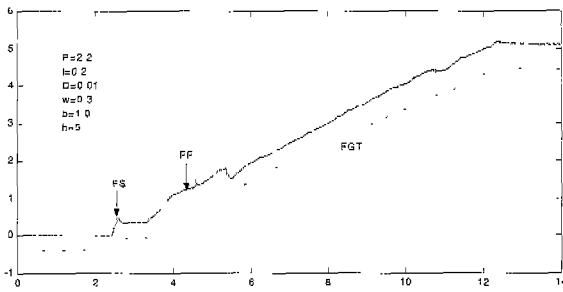
Fig. 30. Fuel loop feedback control by the NN-Tuning 2-DOF PID controller during a gas temperature disturbance ( P=2.2 , I=0.2 , D=0.01 , w=0.3 , b=1.0 , h=5 ).
