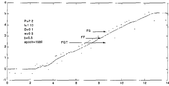
Fig. 19. Fuel loop feedback control by the NN-Tuning 2-DOF PID controller ( P=2.2 , I=1.1 , D=0.1 , w=0.8 , b=0.9 , epoch=1000).
