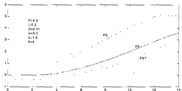
Fig. 29. Fuel loop feedback control by the NN-Tuning 2-DOF PID controller during a gas temperature disturbance ( P=2.2 , I=0.2 , D=0.01 , w=0.5 , b=1.5 , h=8 ).
