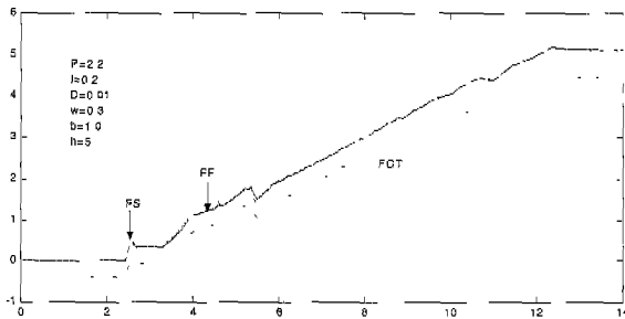
Fig. 24. Fuel loop feedback control by the NN-Tuning 2-DOF PID controller ( P=2.2 , I=0.2 , D=0.01 , w=0.3 , b=1.0 , h=5 ).
