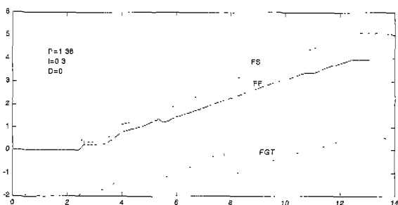
Fig. 11. Fuel loop feedback control by the PID controller in gas temperature disturbance (P=1.38, I=0.3, D=0).
