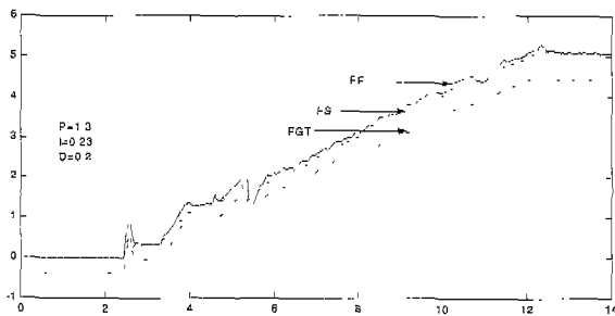
Fig. 10. Fuel loop feedback control by the PID controller (P=1.3, I=0.23, D=0.2).
