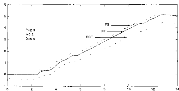
Fig. 9. Fuel loop feedback control by the PID controller ( P=2.3 , I=0.2 , D=0 ).
