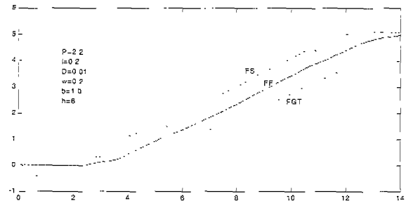
Fig. 28. Fuel loop feedback control by the NN-Tuning 2-DOF PID controller during a gas temperature disturbance ( P=2.2 , I=0.2 , D=0.01 , w=0.2 , b=1.0 , h=8 ).
