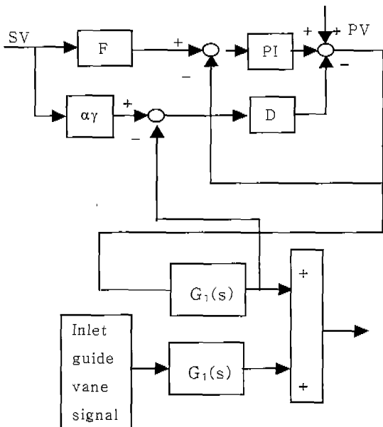
Fig. 3. The structure of the 2-DOF PID controller with a combined 2-DOF parameter for the Gun-san gas turbine
