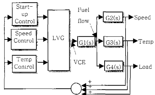
Fig. 2. Control system of the Gun-san gas turbine generating plant: VCE=fuel flow signal, G1(s)= transfer function of fuel system, G2(s)=transfer function of between fuel flow and turbine speed, G3(s)=transfer function of between fuel flow and turbine exhaust gas temperature, G4(s)=transfer function of between fuel flow and generator output.
