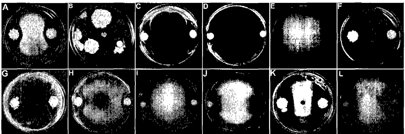
Fig. 1. Antifungal spectrum of Bacillus subtilis YS1.
