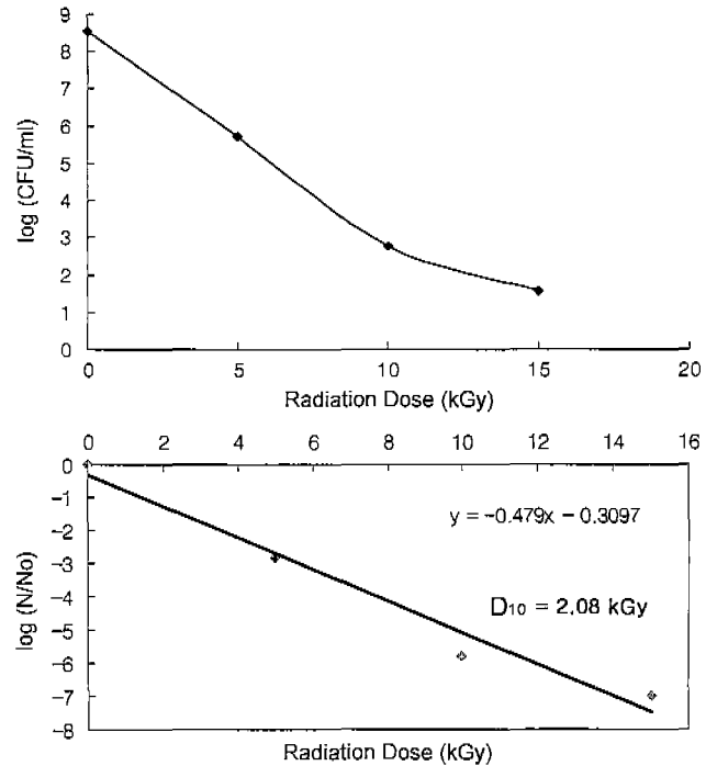
Fig. 2. Radiation sensitivity of Bacillus subtilis YS1 isolated from hot spring. D_{10} value is -1/\text{slope} .
