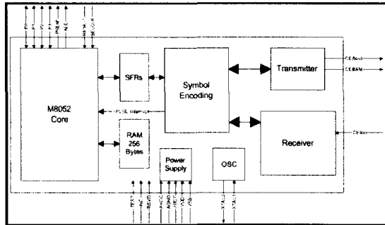
Fig. 6 Architecture of PLC controller
