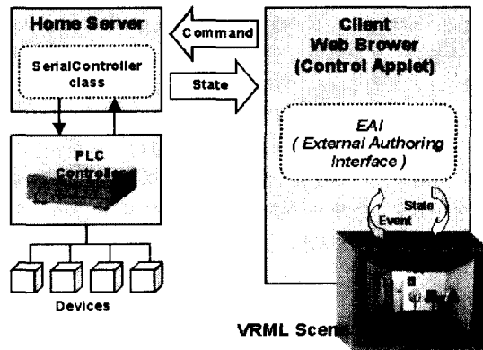
Fig. 4 Operating method of EAI (External Authoring Interface)
