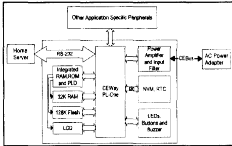
Fig. 7 Interface diagram of PLC controller
