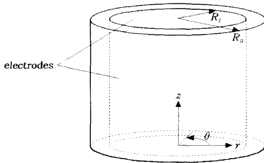
Fig. 1 Schematic diagram of a cylindrical transducer.
