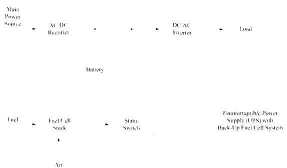
Fig. 20. Block diagram of a UPS with back-up fuel cell system
