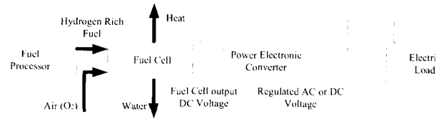
Fig. 9. Block diagram of a typical fuel cell based power processing system
