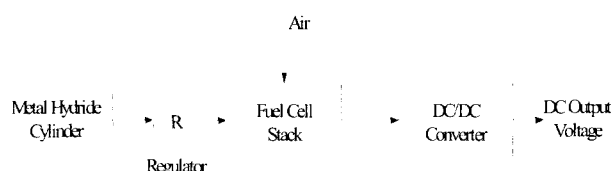
Fig. 18. Block diagram of a PAFC based portable power unit
