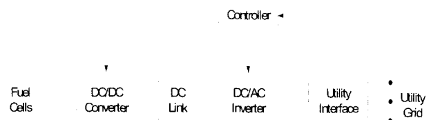
Fig. 11. Block diagram of a typical fuel cell based generation system for utility applications.
