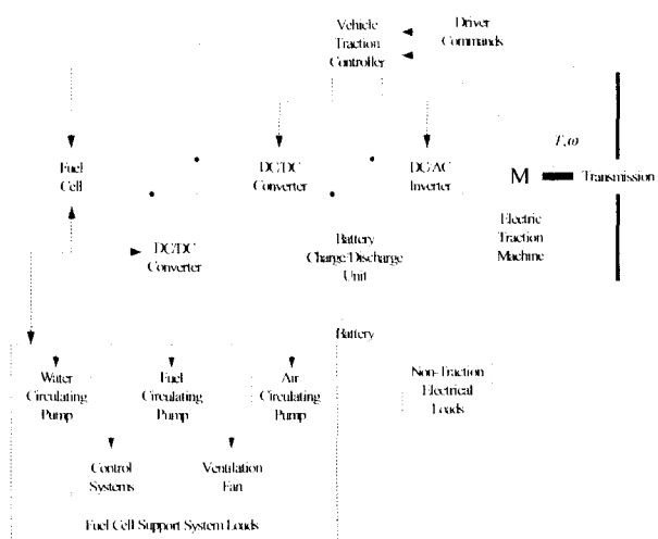
Fig. 13. Power system of an automobile with a fuel cell based drive train
