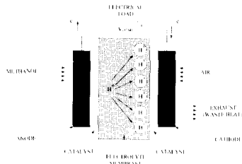
Fig. 7. Schematic diagram of a typical DMFC
