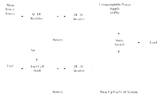
Fig. 19. Block diagram of a fuel cell back-up power supply
