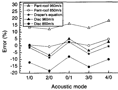
Fig. 2 Calculation error correlation between Draper's equation and FEM analysis
