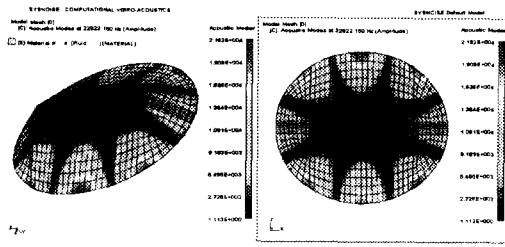
Fig. 11 Acoustic mode shape in the pent-roof combustion chamber(4/0 mode, 22822Hz)
