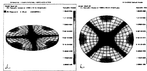
Fig. 4 Acoustic mode shape in the equivalent combustion chamber(2/0 mode, 12663Hz)
