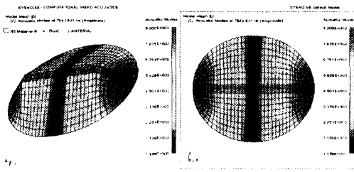
Fig. 5 Acoustic mode shape in the pent-roof combustion chamber(1/0 mode, 7644Hz)
