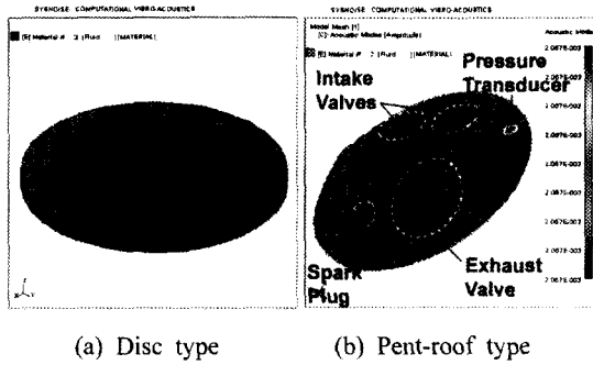
Fig. 1 FEM Model of the Combustion Chamber
