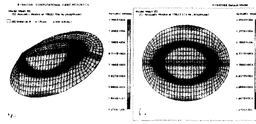
Fig. 8 Acoustic mode shape in the pent-roof combustion chamber(0/1 mode, 15624Hz)
