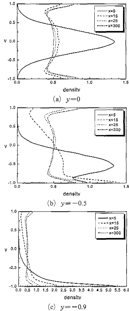
Fig. 5 Distribution of particles in the x-y plane continuously released at: (a) Y(0)=0 ; (b) Y(0)=-0.5
