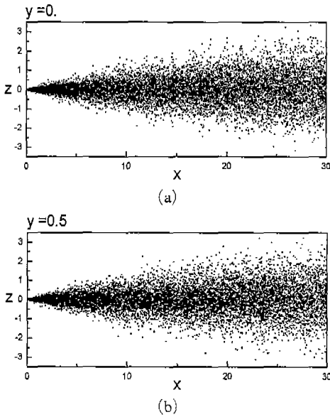
Fig. 4 \eta of Eq. (18) (a) in the wall-normal and (b) in the spanwise direction
