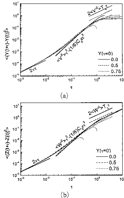
Fig. 1 Dispersion in the wall-normal and spanwise direction of particles released at three different initial locations
