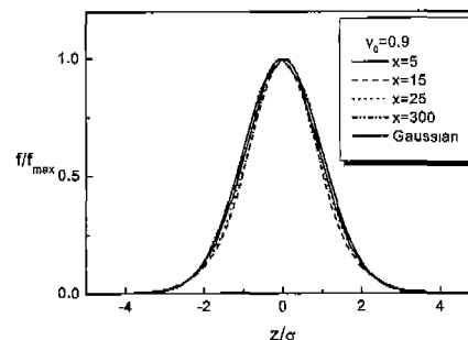
Fig. 8 Probability density distribution of particle's position in the spanwise direction at several downstream locations
