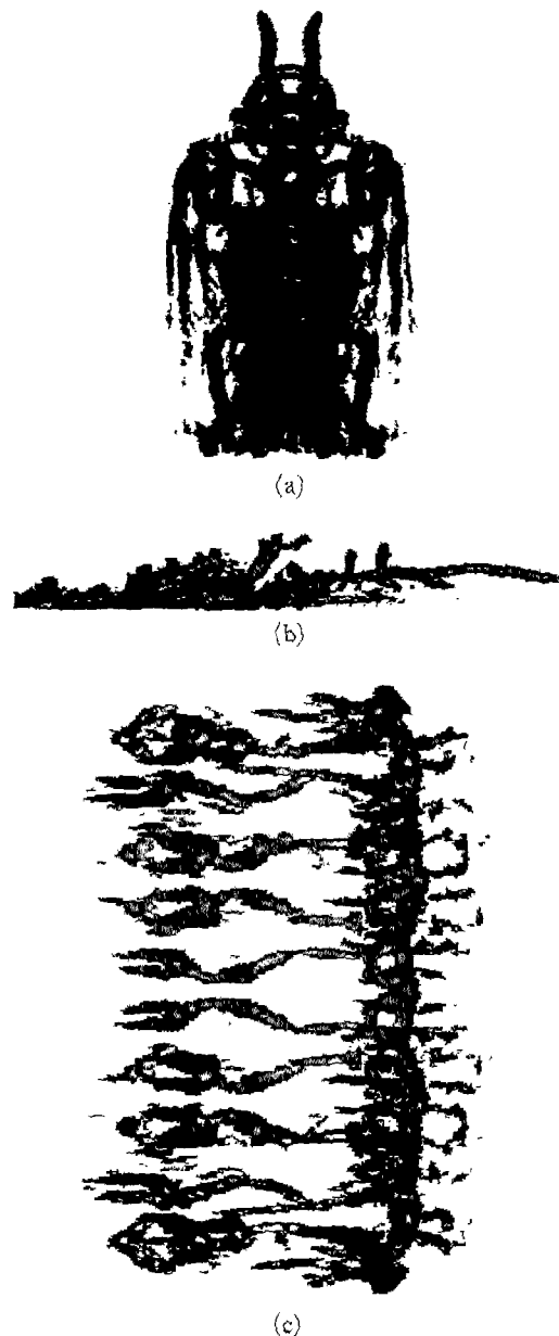
Fig. 8 Interactions of multiple hairpin packets in a mean turbulent flow at Re_\tau \approx 300 . (a) and (b) are the perspective and side views of the vortical structure resulting from interactions of five hairpins, four of them are located at each corner of a rectangle and one in the center of it. (c) is the top view of ten interacting hairpins aligned in the lateral direction. After pairing the ten hairpins form five groups, each of them developed from spanwise interaction
