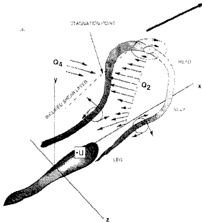
Fig. 1 Paradigm of a single hairpin vortex
