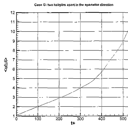
Fig. 7 After the lateral encounter of two hairpins the kinetic energy of the streamwise velocity increases more rapidly as a result of a reduction of back-induction by the hairpins
