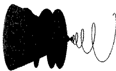
unstable focus
