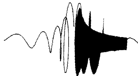
saddle-spiral
