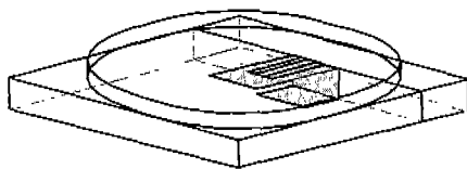
Fig. 4 Schematic illustration of the manganin pressure gauge (Upper plate was used as the stress medium, and lower plate was used to protect and fix the gauge)
