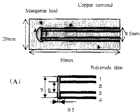
Fig. 3 Detail illustrations of manganin gauge (The manganin foil of between the second terminal and the third terminal is the pressure measurement section)
