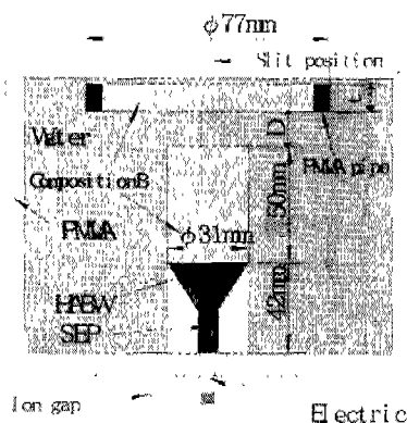
Fig. 1 Schematic diagram of optical observation device used in the experiment of underwater sympathetic detonation
