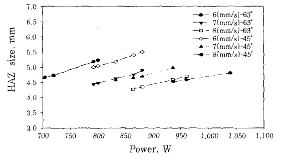
(a) HAZ size at the pipe
