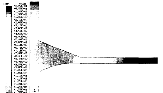
(b) The mid step after filled with filler metal
