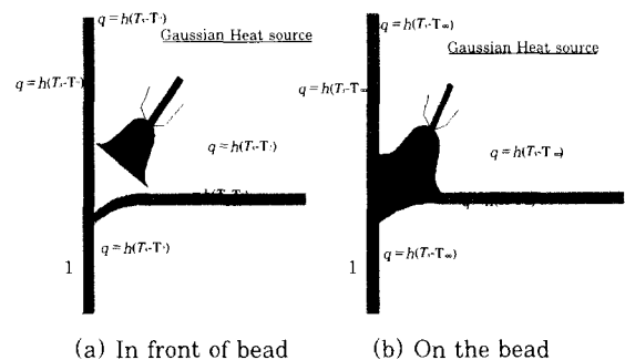
Fig. 2 Boundary conditions for thermal analysis
