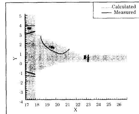
Fig. 10 Comparison of the calculated and measured HAZ size (100A, 16V : 6mm/s)
