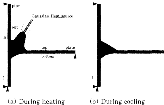
Fig. 3 Boundary conditions for stress analysis
