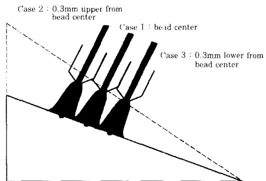
Fig. 4 Cases of torch position
