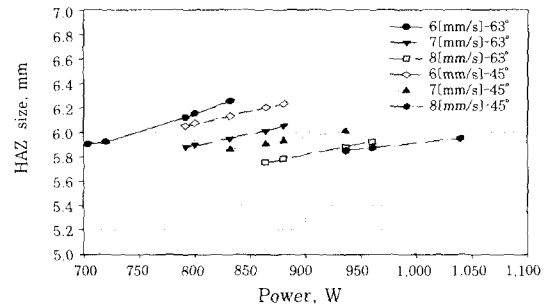
(b) HAZ size at the plate
