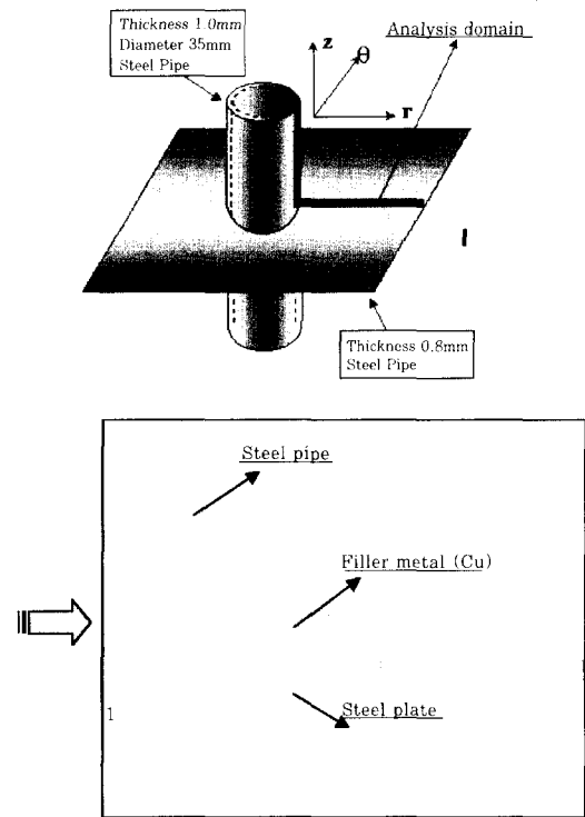
Fig. 1 Schematic of solution domain
