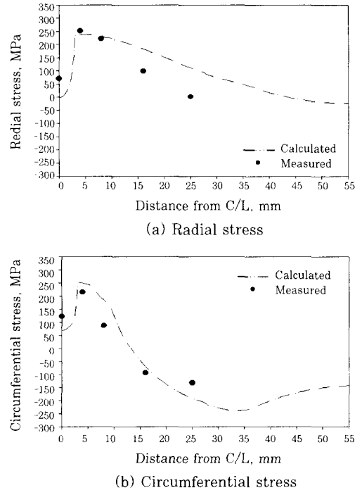
Fig. 20 Comparison of calculated residual stresses with measured one on the top surface of plate ( 100A, 16V, 6mm/s )
