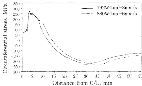
Fig. 22 Circumferential stress distributions according to traveling speed and power on the top surface of plate
