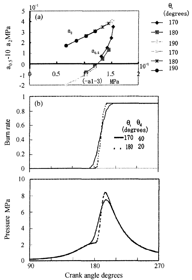
Figure 4. (a) Relationship between Fourier series, (b) Traces of burn rate and pressure.
