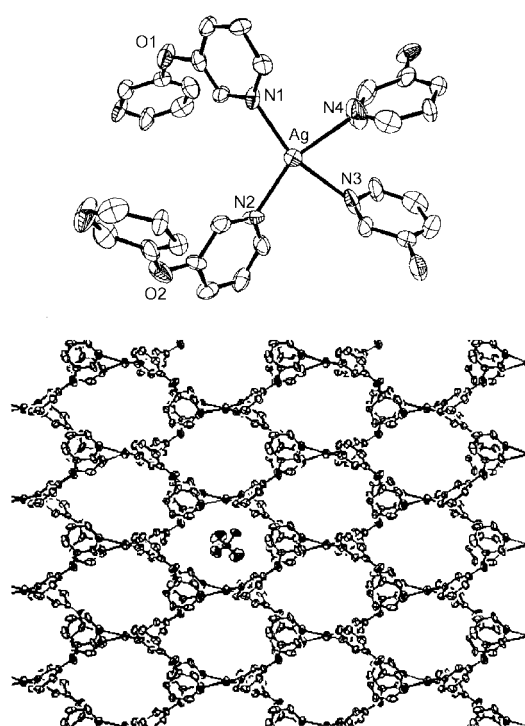
Figure 1. Asymmetric unit (up) and infinite network structure (down) of [\text{Ag}(\text{Py}_2\text{O})_2]\text{BF}_4 . Only a counteranion was presented for clarity.
