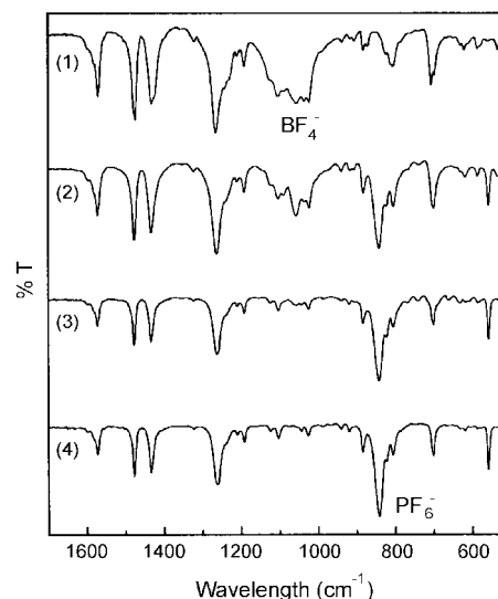
Figure 2. (a) IR (KBr pellet) change procedure during the counteranion exchange of [\text{Ag}(\text{Py}_2\text{O})_2]\text{BF}_4 with \text{NaPF}_6 . (1) [\text{Ag}(\text{Py}_2\text{O})_2]\text{BF}_4 (2) after 6 h, (3) after 12 h, and (4) after 24 h.
