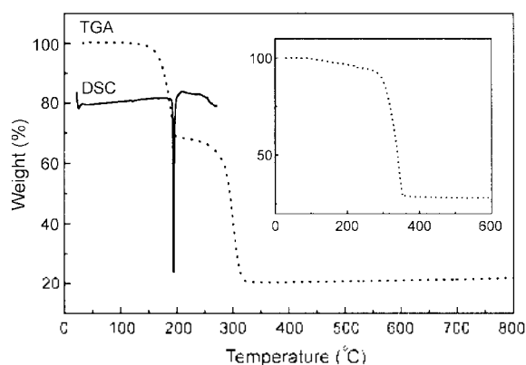
Figure 3. Overlay of TGA and DSC traces of [\text{Ag}(\text{Py}_2\text{O})_2]\text{BF}_4 , each recorded at heating rate of 5\text{ °C min}^{-1} . The TGA curve in box was taken on the helical structure, [\text{Ag}(\text{Py}_2\text{O})]\text{BF}_4 .
