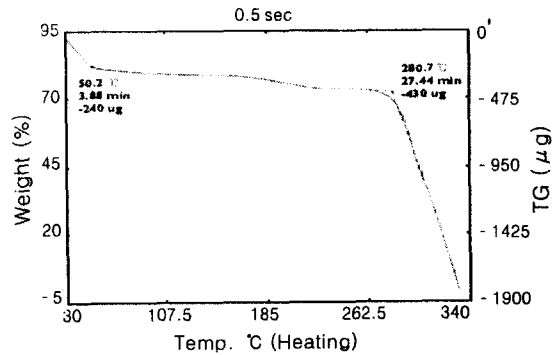
Figure 3. TGA thermogram of NLO-polyquinonediimine (di-azobenzene).
