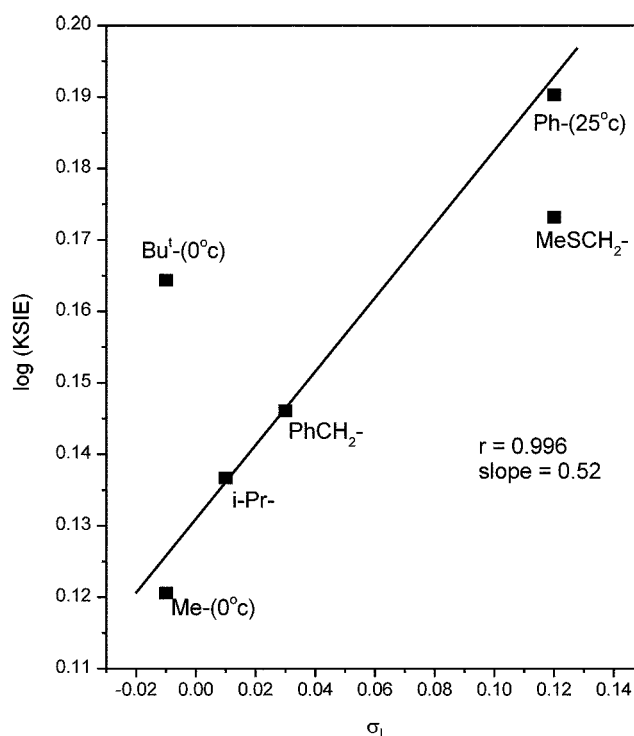
Figure 5. Plot of \log(\text{KSIE}) in methanol vs inductive parameter ( \sigma_I ) for substituted acetyl chloride at 10 °C [(removed two point (Bu - and MeSCH 2 - groups) in correlation)]
