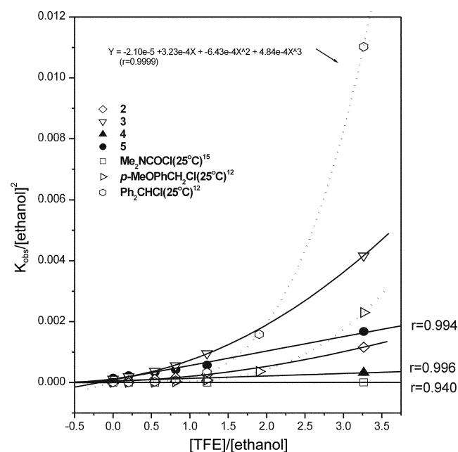
Figure 4. Plots of K_{obs}/[\text{ethanol}]^2 vs. molar ratio of TFE and ethanol for solvolysis of various substrates in TFE-ethanol mixture at 10 °C.
