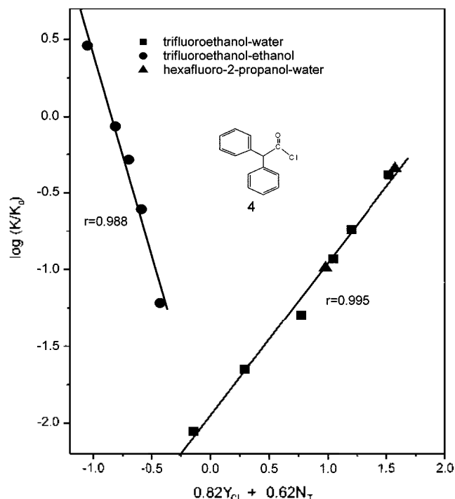
Figure 2. Plots of \log(K/K_0) for solvolyses of rdiphenylacetyl chloride ( 4 ) at 10 °C against (0.82 Y_{Cl} + 0.62 N_T) . The five values for solvolyses in TFE-ethanol are not included in the correlation.
