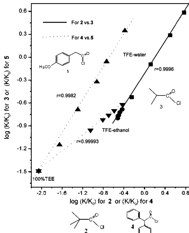
Figure 3. Rate-rate profile between solvolyses of compounds studied in TFE-water and TFE-ethanol mixtures at 10 °C.
