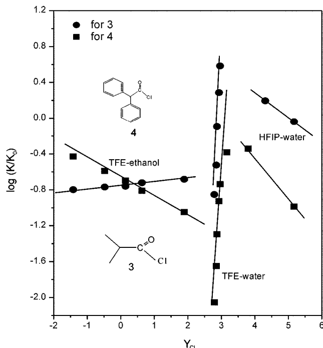
Figure 1. Grunwald-winstein plot for solvolyses of 3 and 4 compounds in various fluorinated solvent mixtures at 10 °C ( m = 8.58 , c = -24.82 for 3 and m = 4.37 , c = -13.95 for 4 in TFE-water)
