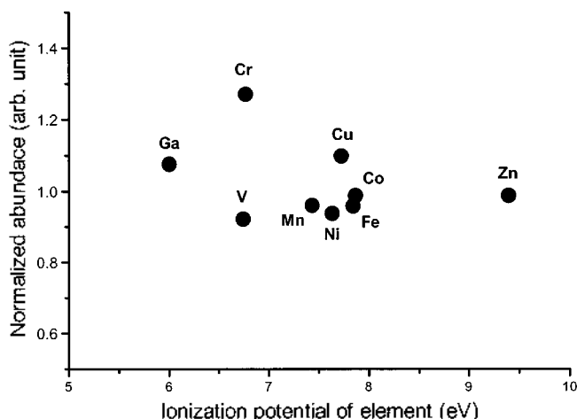
Figure 4. Normalized abundance of elements in 1% CH 3 OH.
