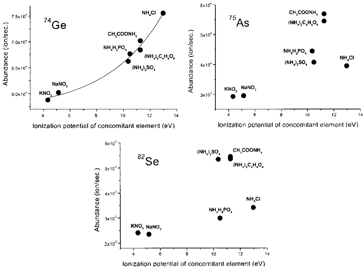
Figure 3. The effect of the concomitant elements on the abundance of Ge, As and Se.
