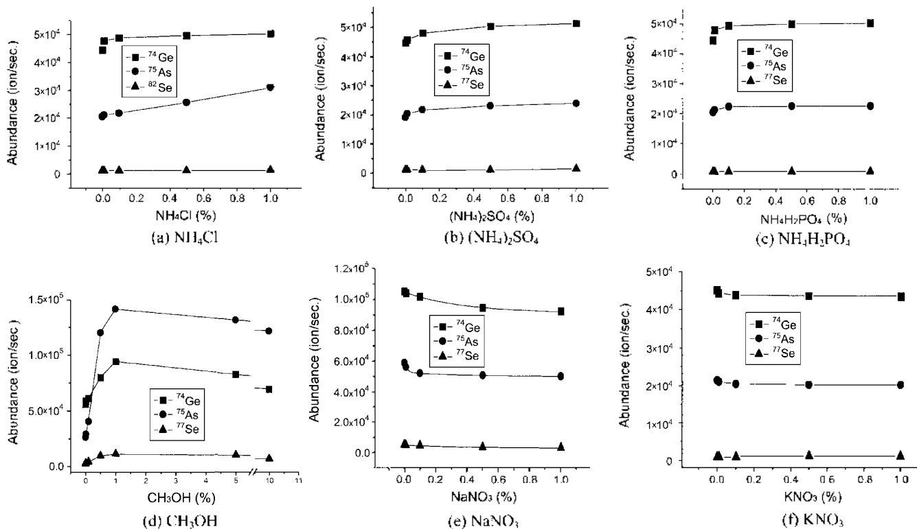
Figure 2. The effect of some matrix concentrations on the abundance of Ge, As and Se.
