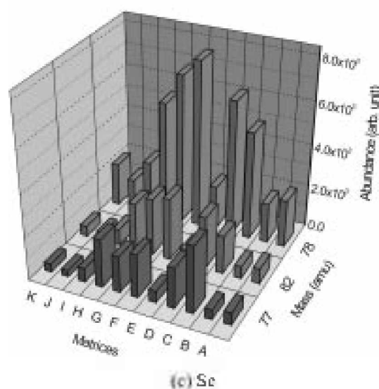
Figure 1. The signal intensity of three elements in various matrices: A: H 2 O, B: HNO 3 , C: HCl, D: H 2 SO 4 , E: H 3 PO 4 , F: CH 3 OH, G: C 2 H 5 OH, H: Mannitol, I: NH 4 OH, J: NaOH, K: KOH.
