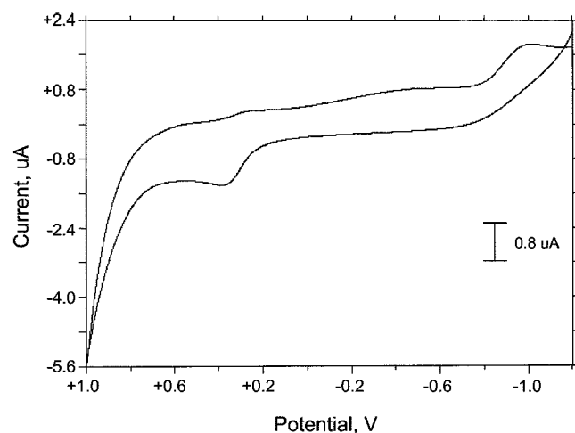
Figure 4. Cyclic voltammogram of [Ni(L)(INT) 2 ]-5H 2 O ( 1 ) in 0.01 M TFAP-DMSO solution at 20.0 ± 0.1 °C. The scan rate is 50 mV/s.
