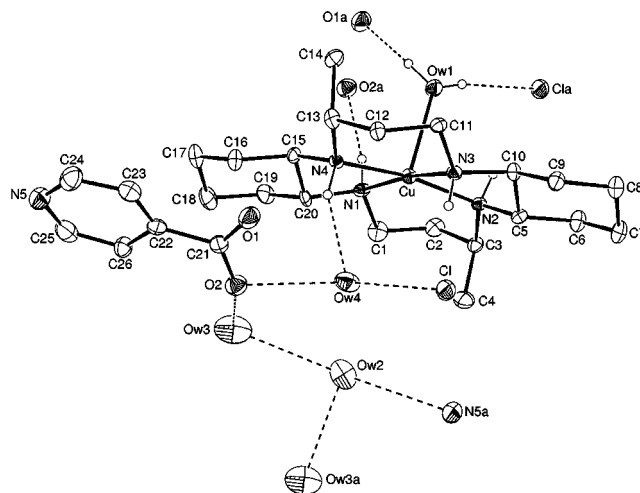
Figure 2. An ORTEP drawing of [\text{Cu}(\text{L})(1\text{L}_2\text{O})](\text{Cl})(\text{INT}) \cdot 3\text{H}_2\text{O} ( 2 ) with the atomic labelling scheme (30% probability ellipsoids shown). The dotted lines indicate the hydrogen bonds.
