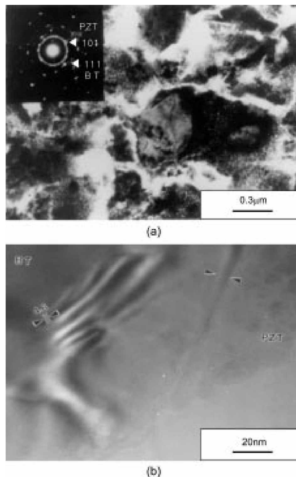
Figure 9. TEM image and diffraction pattern of BT seeded PZT powders. (a) low magnification image with diffraction pattern, (b) high magnification image of the interface between BT seed and PZT.
