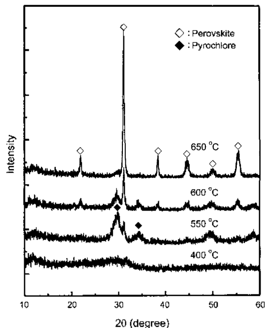
Figure 3. XRD patterns of unseeded PZT powders heated at various temperature for 1 hour.
