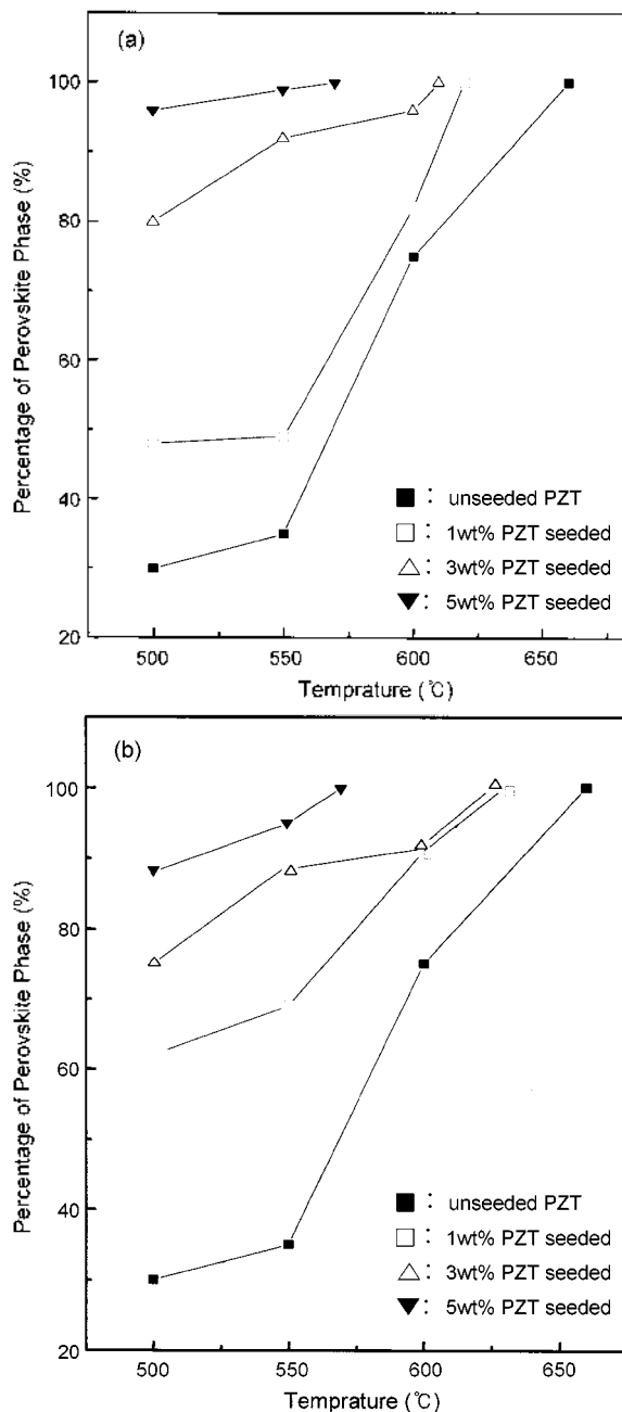
Figure 6. Percentage of perovskite phase vs. temperature for the seeded PZT with various concentration of 1.2 \mu\text{m} (a) PZT and (b) BT seed.
