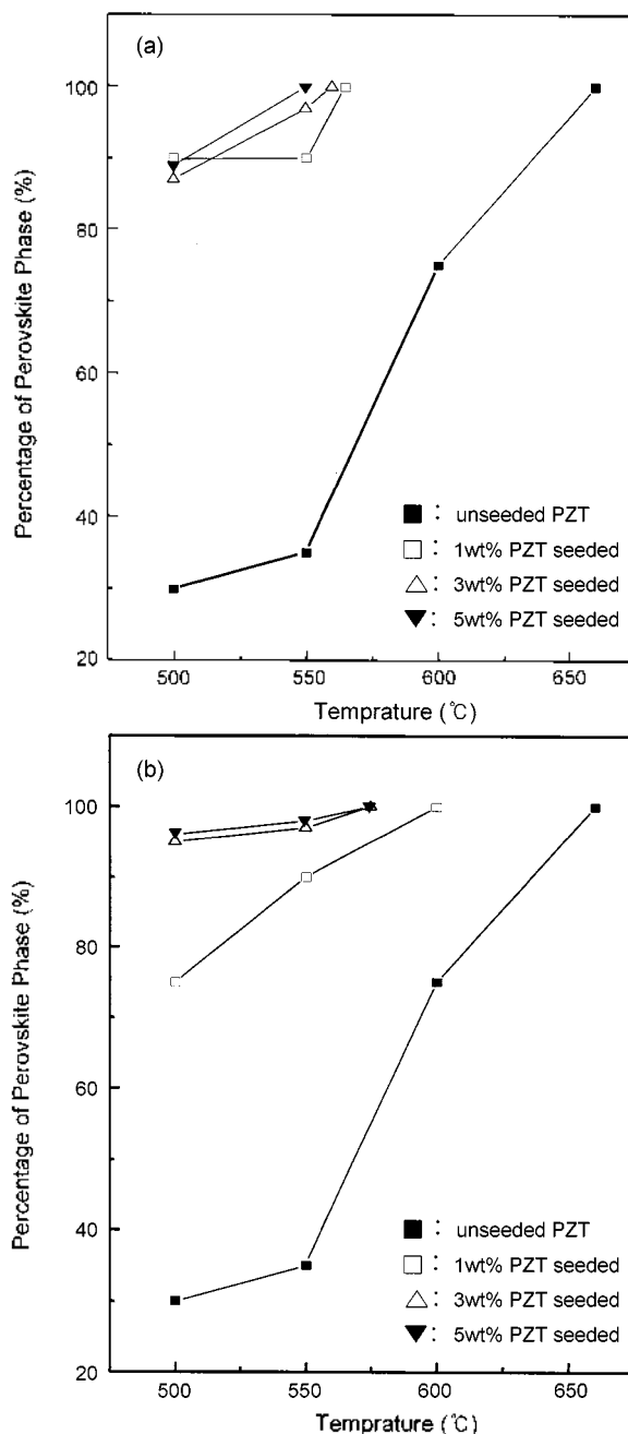
Figure 5. Percentage of perovskite phase vs. temperature for the seeded PZT with various concentration of 0.2 \mu\text{m} (a) PZT and (b) BT seed.
