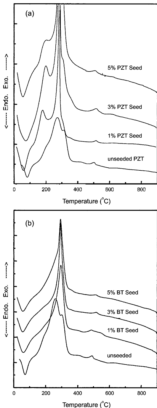
Figure 2. DTA curves of PZT gel powder seeded with various amounts of 1.2 \mu\text{m} size (a) PZT and (b) BT seed.
