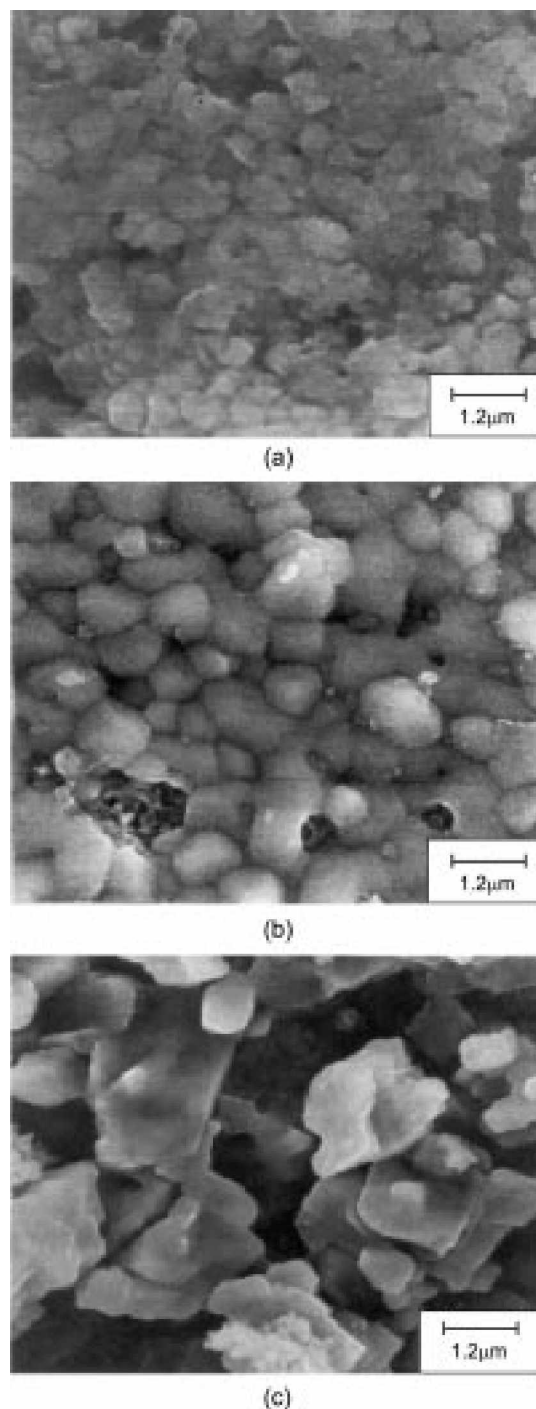
Figure 8. Microstructure of seeded PZT powder with various amounts of BT calcined at 600 °C for 4 hours. (a) 1 wt%, (b) 3 wt%, (c) 5 wt%.
