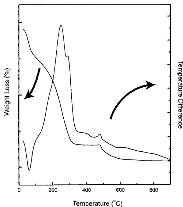
Figure 1. DTA and TGA curves for the unseeded PZT gel powder.
