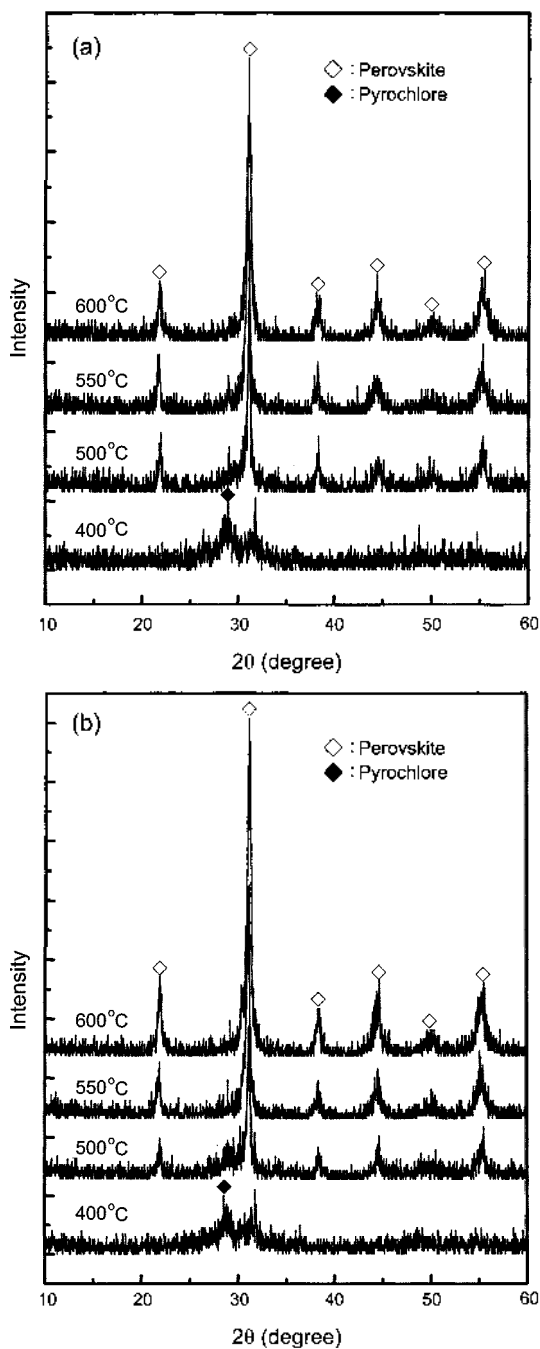
Figure 4. XRD patterns of PZT powders seeded with 3 wt% (a) PZT and (b) BT seed ( 0.2 \mu\text{m} ) heated at various temperature for 1 hour.
