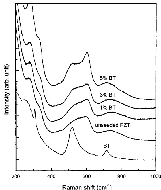
Figure 7. Raman spectra of seeded PZT powders with various concentration of BT seed.
