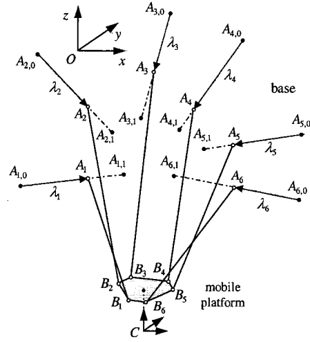
Fig. 2 Schematic diagram of hexaSlide manipulator
