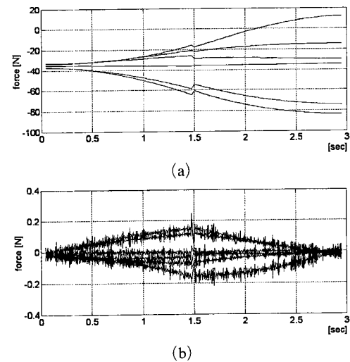
Fig. 8 (a) Actuator forces from DADS and MATLAB for a sample desired trajectory of the platform that is moving with a constant acceleration, (b) Discrepancy between the actuator forces from DADS and MATLAB
