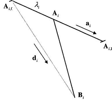
Fig. 3 Kinematic model of slider and link
