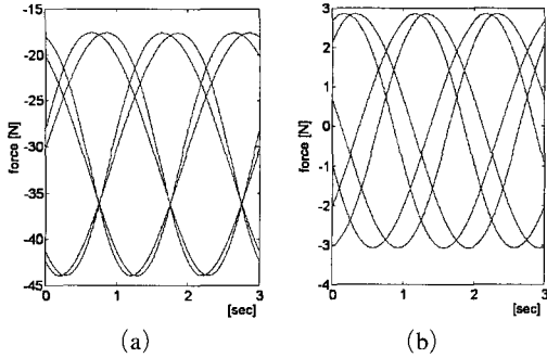
Fig. 9 Total actuator (a) and link inertia actuator force (b) (speed=20 rpm)
