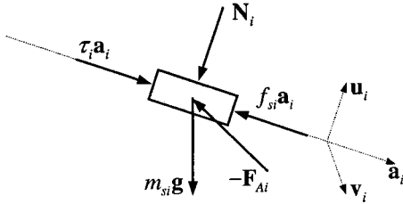
Fig. 4 The detailed dynamic model of slider part
