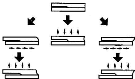
Fig. 3 Applied loading condition at specimen
