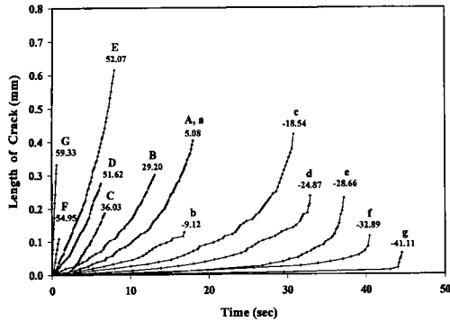
Fig. 9 Behavior of interfacial crack propagation with mode-mix
