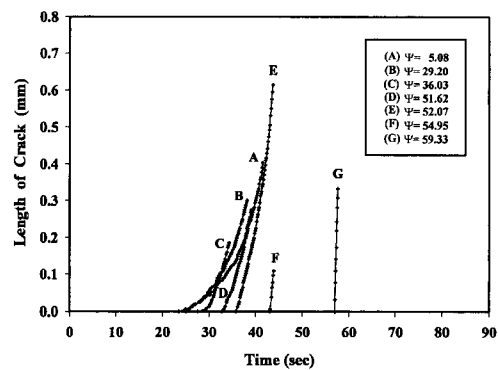
Fig. 7 Behavior of interfacial crack propagation under positive mode-mix
