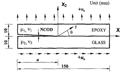
Fig. 1 Bimaterial edge-cracked strip specimen
