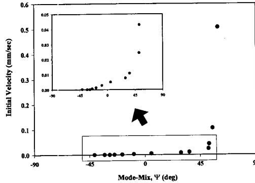
Fig. 12 Initial velocity of crack propagation with mode-mix
