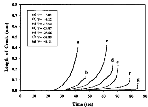
Fig. 8 Behavior of interfacial crack propagation under negative mode-mix
