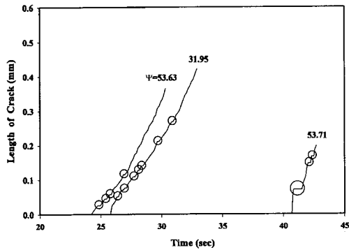
Fig. 10 Stick-slip behavior in interfacial crack propagation
