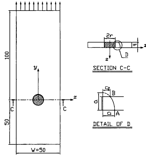
Fig. 5 Configuration of an elliptical arc through crack in a mechanical joint
