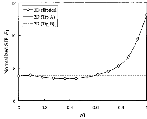
Fig. 18 Comparison of mode I stress intensity factors for elliptical arc through cracks and two-dimensional cracks in mechanical joints
