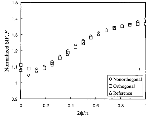
Fig. 11 Stress intensity factors for semi-elliptical surface crack in a finite-width plate using orthogonal and non-orthogonal mesh
