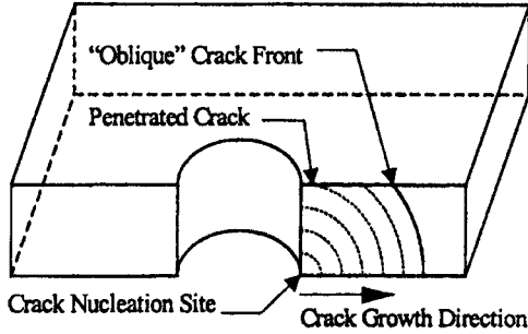
Fig. 1 Crack growth profile in mechanical joints (Fawaz, 1999)
