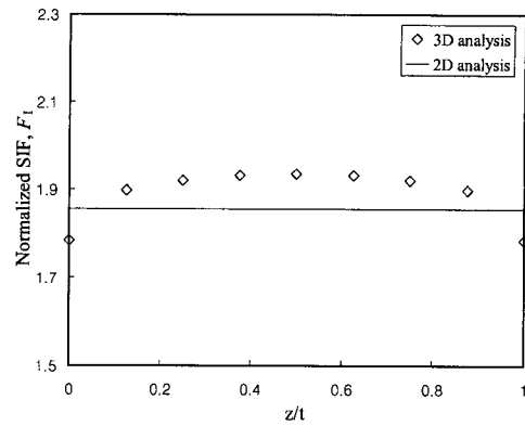
Fig. 14 Stress intensity factors along thickness of a through crack in mechanical joints
