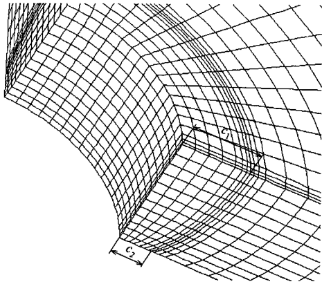
Fig. 12 Finite element mesh for symmetric elliptical arc through cracks at a fastener hole
