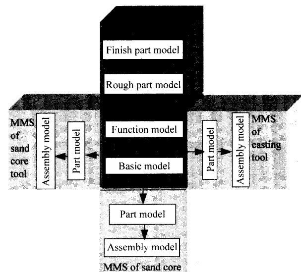
Figure 3. Integrated modeling based on multi model technology.
