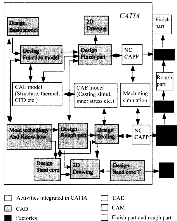
Figure 5. Integration frame of CAD/CAM/CAE in cylinder head development process.
