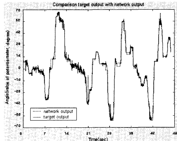
Figure 4. Comparison between network output and target output.
