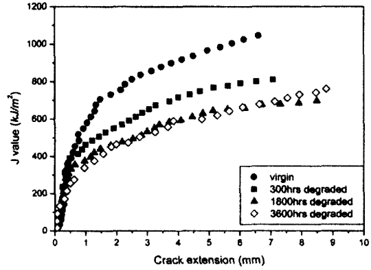
Fig. 3 J - R curves for virgin and degraded specimens
