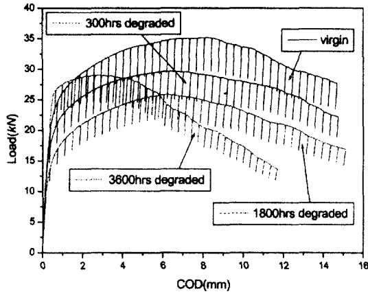
Fig. 2 Load-load line displacement curves
