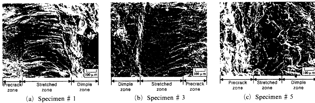
Fig. 5 Fractograph of the virgin specimens in the stretched zone
