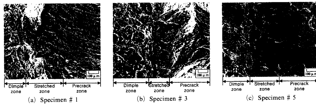
Fig. 7 Fractograph of the 1800hrs. degraded specimens in the stretched zone
