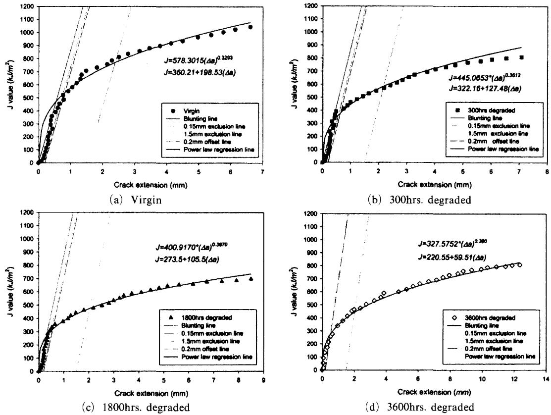
Fig. 4 Determination of J_{IC} by the ASTM E 813-87 method
