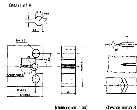
Fig. 1 Geometry of the CT specimen
