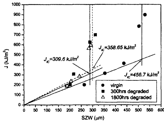
Fig. 8 Determination of the J_{IC} for virgin and degraded specimens by the SZW method
