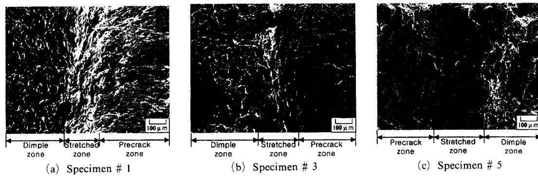
Fig. 6 Fractograph of the 300hrs. degraded specimens in the stretched zone
