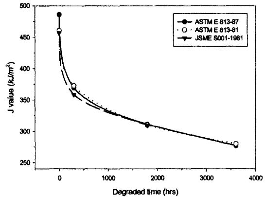
Fig. 9 Relationship between the ASTM E 813-87, the ASTM E 813-81, and the JSME S 001-1981 SZW method for the J_{IC}
