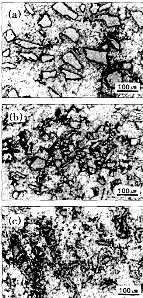
Fig. 2 Optical micrographs of SiCp/AC8A composite with various particle sizes : (a) 100 \mu m, (b) 38 \mu m and (c) 26 \mu m SiC particle reinforced composite.
