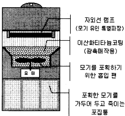
Fig. 4 Schematic drawing of mosquito trap
