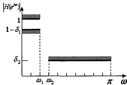
(a) LPF
