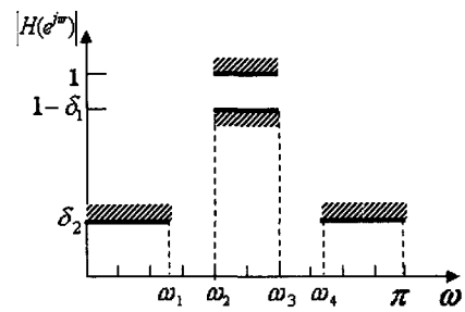
(c) BPF
