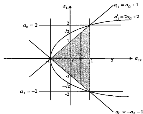
Figure A-1: Region of the filter coefficients that guarantees stability of the second-order IIR filter (the stability triangle)
