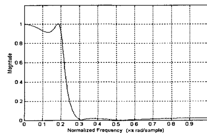
(a) Magnitude response
