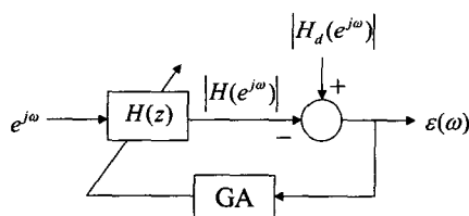
Figure 1: IIR digital filter design using the GA.
