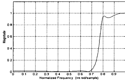
(a) Magnitude response
