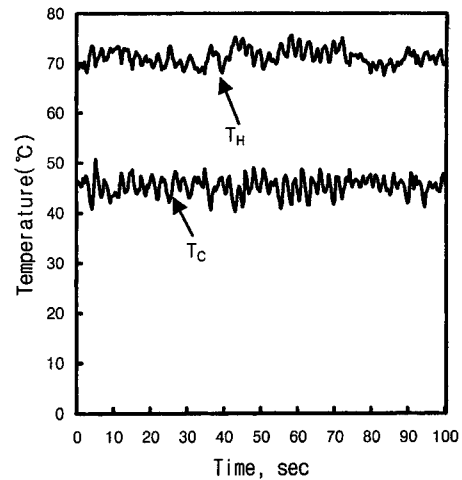
Fig. 3 Temperatures of the heating and the cooling sections
