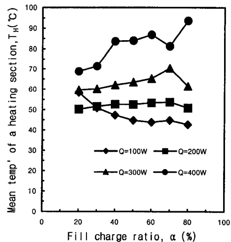
Fig. 4 Mean temperatures of the heating section versus fill charge ratio
