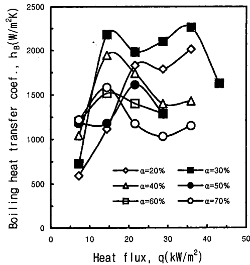
Fig. 8 Boiling heat transfer coefficients of the heat pipe versus heat flux
