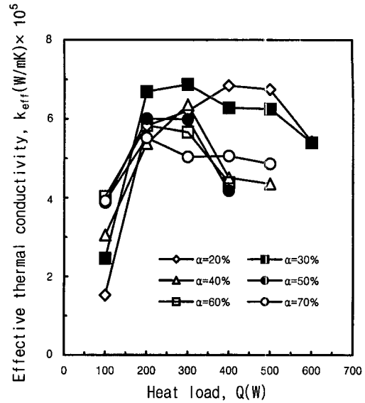
Fig. 7 Effective thermal conductivity of the heat pipe versus heat load
