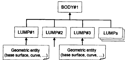
Fig. 5. Data structure after One-Part generation.
