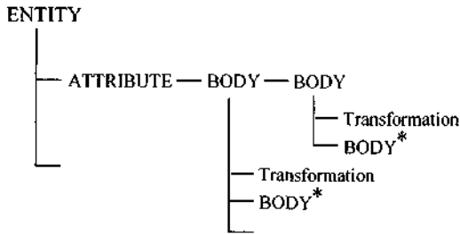
Fig. 3. ACIS data structure after reading a STEP file.
