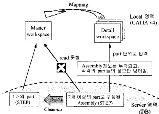
Fig. 1. CAD data flow between Pro/E and CATIA according to STEP AP214.
