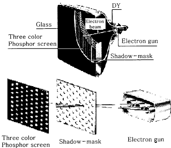
Fig. 1 Structure of braun tube
