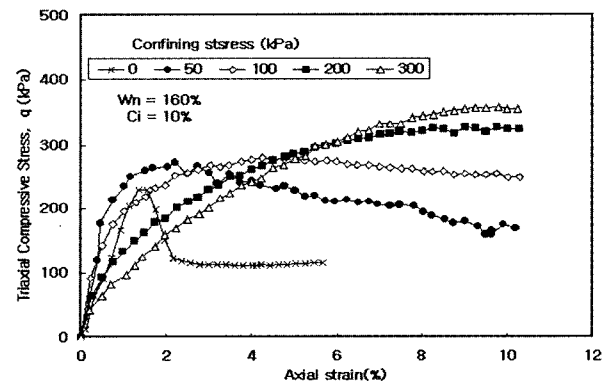
(b) ci=10%, Wi=160%
