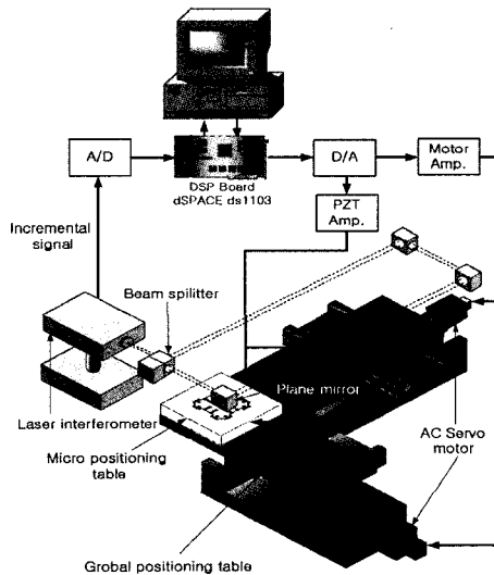
Fig. 3 Schematic diagram of ultra-precision single plane X-Y stage
