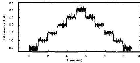
Fig. 13 Resolution experiment of global servo
