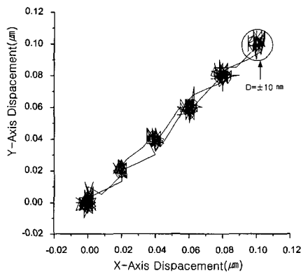
Fig. 19 Resolution experiment of X-Y axis dual positioning control
