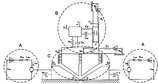
Fig. 1 Modelling of Ultra-precision single plane X-Y stage
