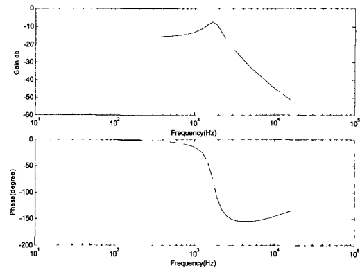
Fig. 8 Bode diagram of micro servo by closed loop for simulation
