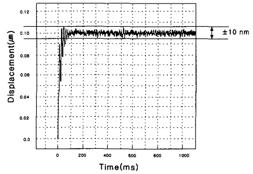
Fig. 14 Step response of micro servo
