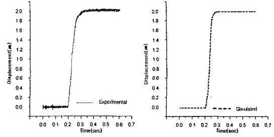
(a) Experiment (b) Simulation
