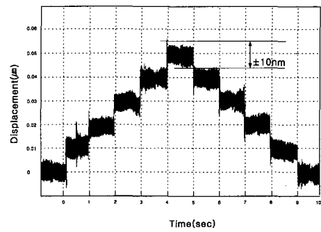
Fig. 16 Resolution experiment of micro servo by closed loop
