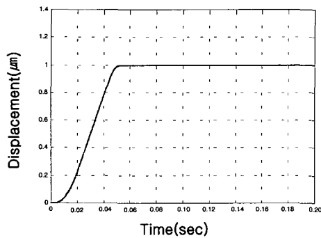
Fig. 7 Step response of global servo for simulation
