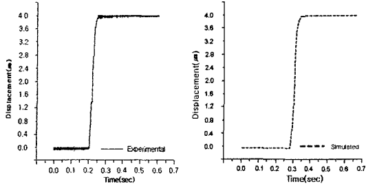
(a) Experiment (b) Simulation
