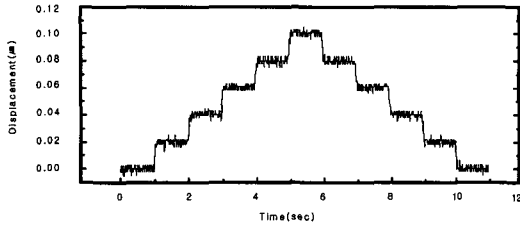
Fig. 17 Resolution experiment of X-axis dual positioning control
