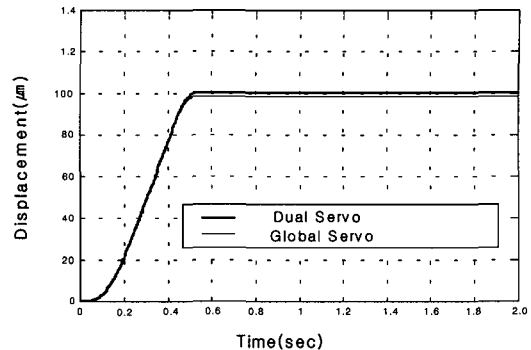
Fig. 10 Step response of dual servo to perform simulation
