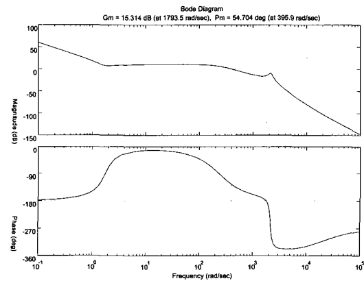
Fig. 6 Bode diagrams of global servo by closed loop for simulation
