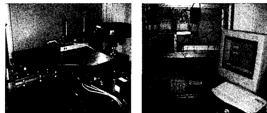
Fig. 4 Photograph of ultra-precision single plane X-Y stage
