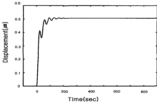
Fig. 9 Step response of micro servo for simulation
