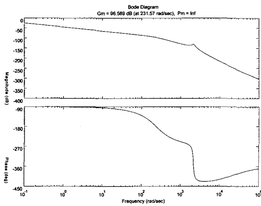
Fig. 5 Bode diagrams of global servo by open loop for simulation
