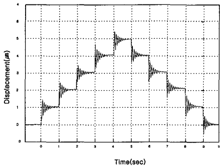
Fig. 15 Resolution experiment of micro servo by open loop
