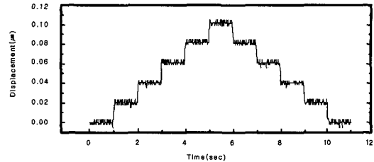
Fig. 18 Resolution experiment of Y-axis dual positioning control
