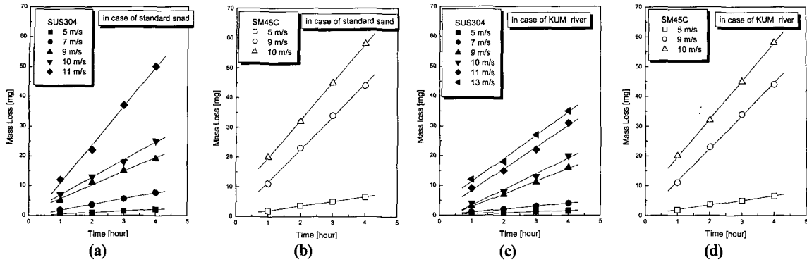
Fig. 3 Mass loss of slurry wear
