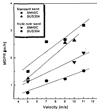
Fig. 7 MDPR with liquid jet velocity
