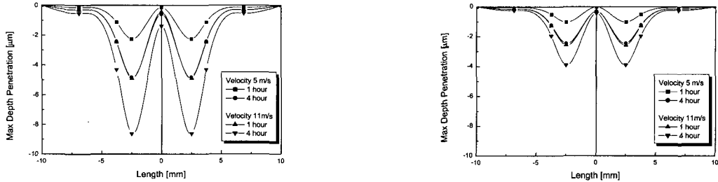
(a) Wear surface with SUS304 in standard sand
