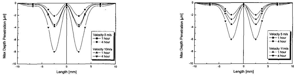
(a) Wear surface with SM45C in standard sand
