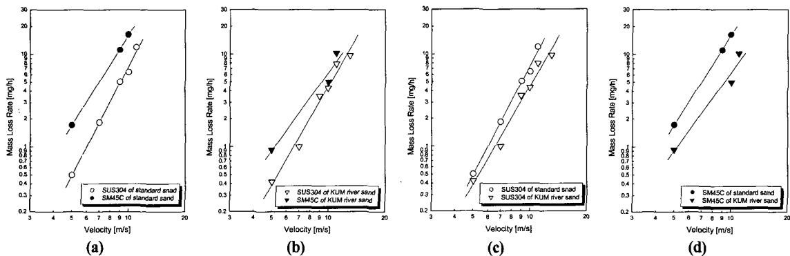
Fig. 4 Mass loss rate of slurry wear
