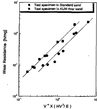
Fig. 8 Wear resistance
