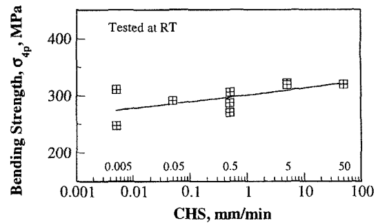
Fig. 3 4-Point bending strength over cross head speeds
