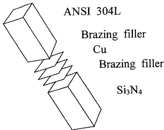
Fig. 1 Specimen configuration
