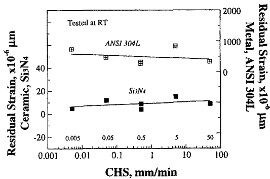
Fig. 6 Residual strain of metal and ceramic as a function of cross head speed
