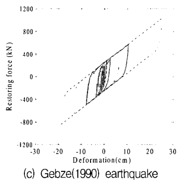
Fig. 8 Restoring force of LRB at pier 2
