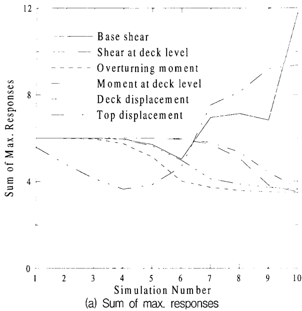
Fig. 5 Selection of appropriate optimal weighting parameters for the active control system
