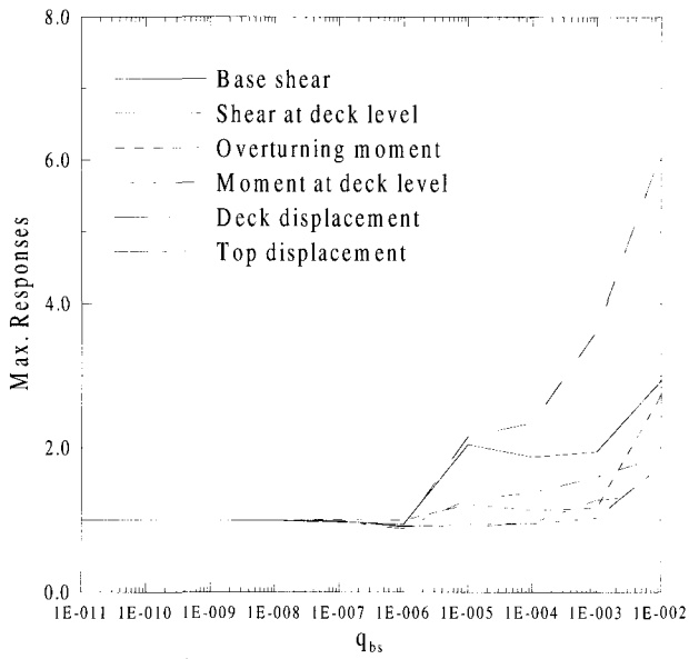
(a) Base shears at piers 2 and 3
