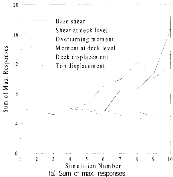
Fig. 7 Selection of appropriate optimal weighting parameters for the hybrid control system
