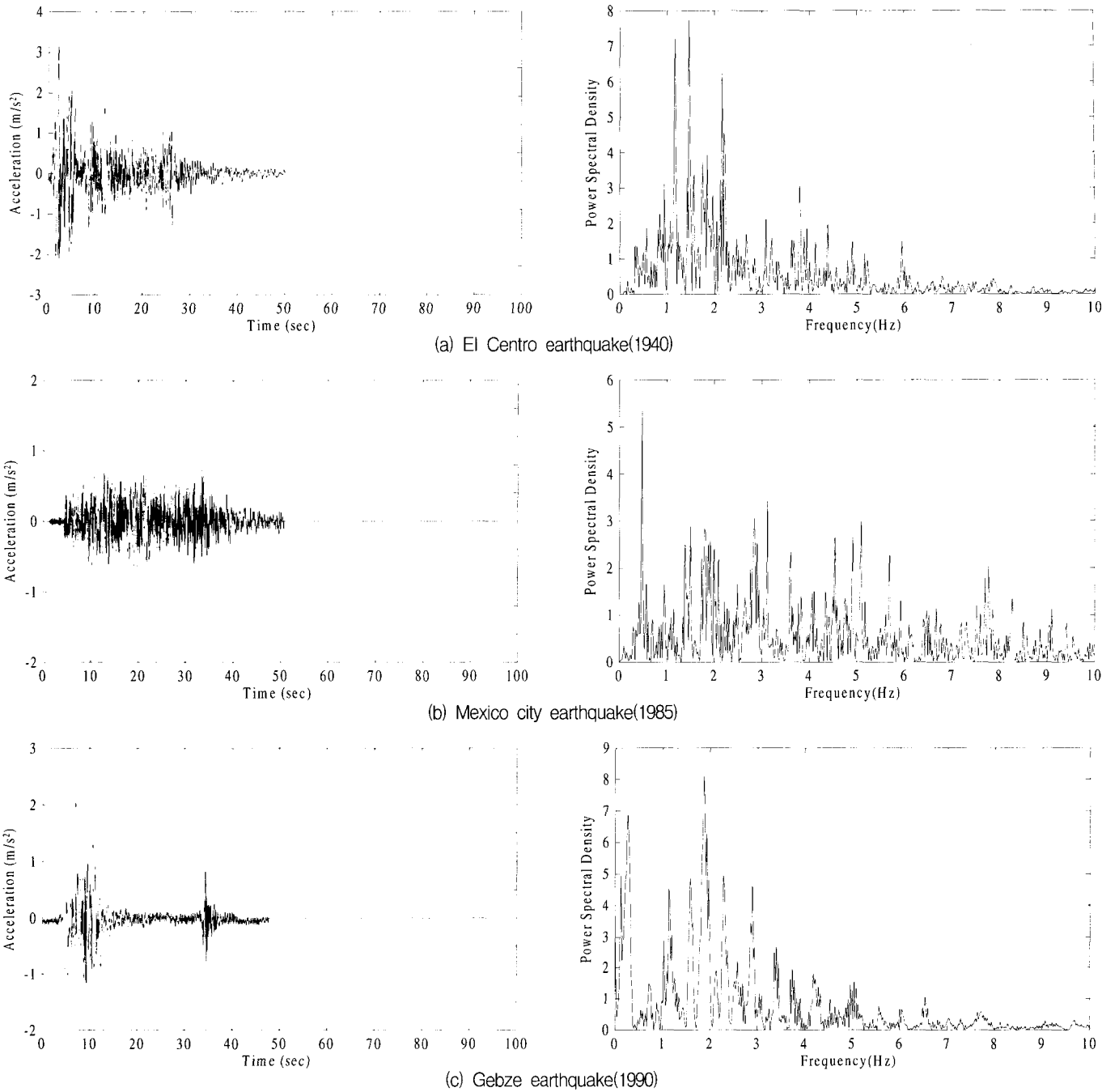
Fig. 3 Time-history and power spectral density of earthquakes
