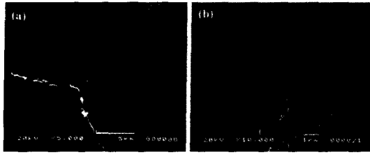
Fig. 8 Precipitate morphology in grain boundary for type 316LN(a) and 9Cr-Mo(b) specimens; 316LN steel is at 300 MPa/600 °C and 9Cr-Mo steel is at 190 MPa/600 °C
