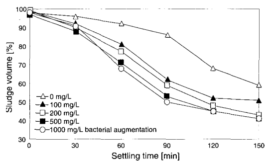
Fig. 4 Effect of concentration of bacterial augmentation with FeSO 4 , 100mg/L.
