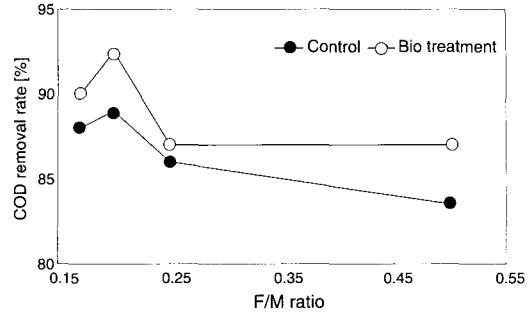
Fig. 2 Variation of COD removal rate on each F/M ratio.
