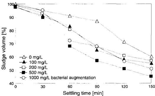
Fig. 3 Effect of concentration of bacterial augmentation with FeCl 3 , 100mg/L.
