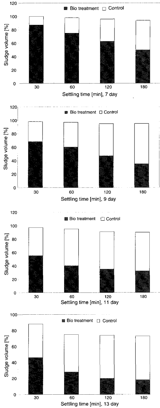
Fig. 6. Variation of sludge volume on the bench scale pilot test.
