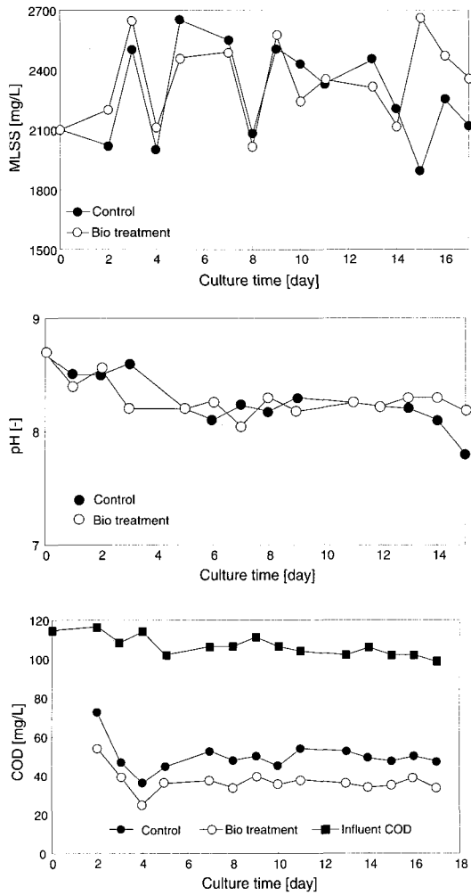
Fig. 5. Continuous treatment in bench scale pilot of food wastewater.
