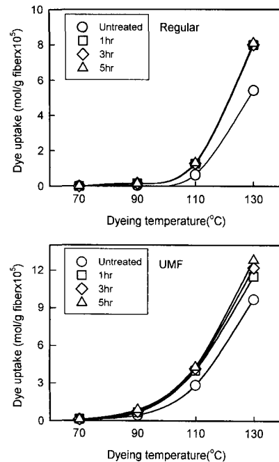
Fig. 2. Relationship between dyeing temperature and dye uptake of Disperse Red 60 on PET regular and UMF filaments treated with DMF at 100°C.
