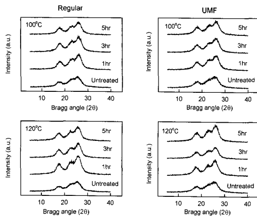
Fig. 3. Wide angle X-ray profiles of PET regular and UMF filaments treated with DMF at 100°C and 120°C.
