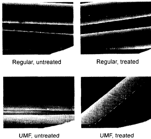
Fig. 8. Scanning electron micrographs of PET regular UMF filaments treated with DMF at 100°C for 1hr.
