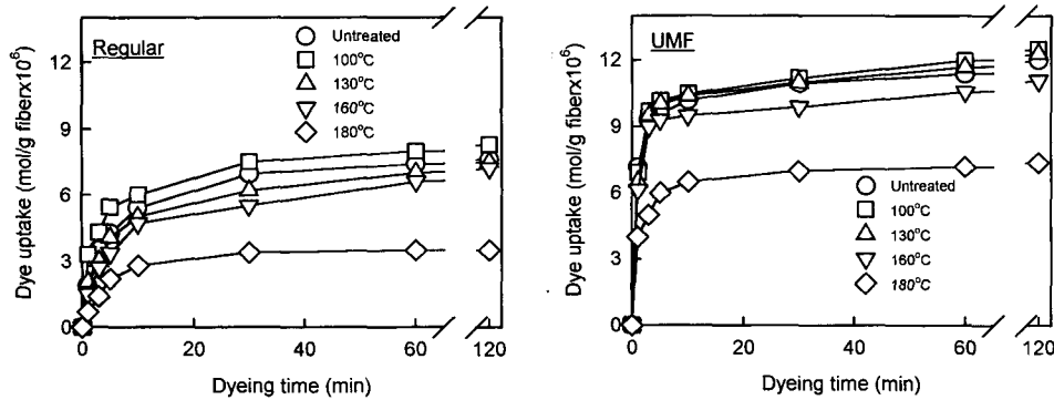
Fig. 1. Dyeing rate of Acid Red 18 on nylon fibers heat-setted for 10 min at various temperatures.
