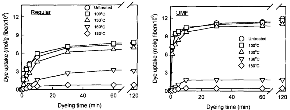
Fig. 2. Dyeing rate of Acid Red 18 on nylon 6 fibers heat-setted for 60 min at various temperatures.
