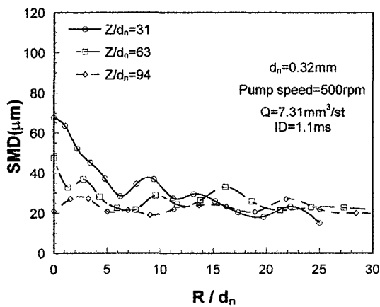
(a) 5-hole nozzle
