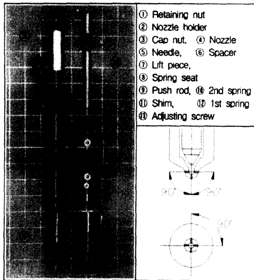
Fig. 2 Photograph of disassembled 5-hole diesel nozzle and schematic diagram of nozzle tip
