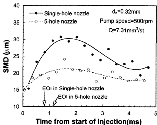
Fig. 10 SMD distribution with time from start of injection, which was calculated with time window of 0.15 ms to all measurement points of spray flow fields
