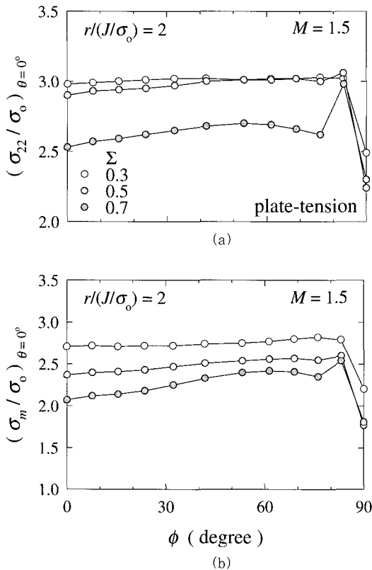
Fig. 6 Normalized (a) crack-tip opening stress and (b) hydrostatic stress along the crack front of plate under remote tension for various load levels
