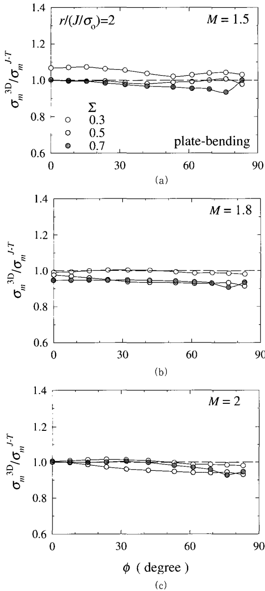
Fig. 15 Hydrostatic stress normalized by J - T solution of plate under remote bending for various plastic strength mismatch
