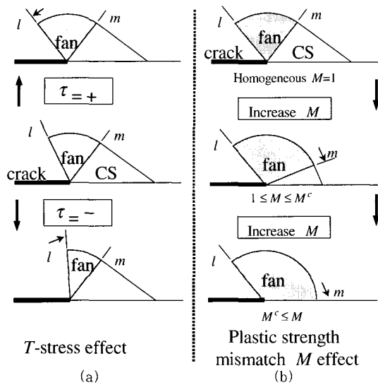
Fig. 8 Schematic slip-line field representation for the effects of (a) T -stress and (b) plastic strength mismatch M
