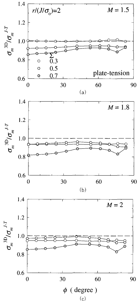
Fig. 14 Hydrostatic stress normalized by J-T solution of plate under remote tension for various plastic strength mismatch
