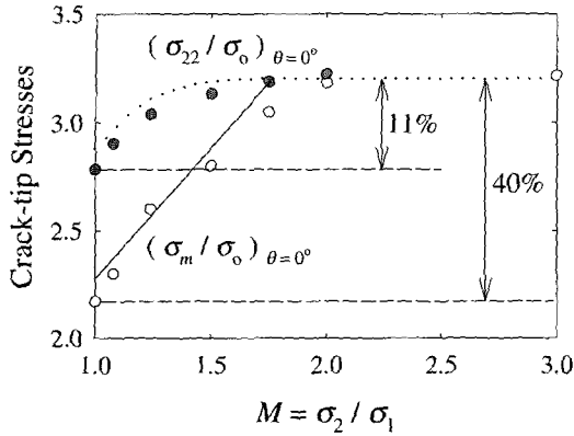
Fig. 12 Variation of the hydrostatic stress and the tensile stress at the interface, (\sigma_m|_{\theta=0^\circ}/\sigma_0) and (\sigma_{22}|_{\theta=0^\circ}/\sigma_0) with plastic strength mismatch M for \tau \equiv T/\sigma_0 = 0
