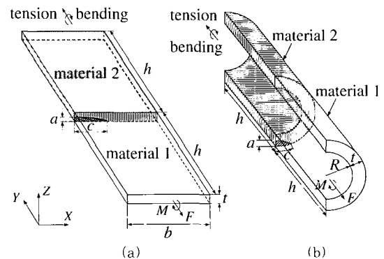
Fig. 1 Schematic diagram of half of elliptical interfacial cracked bimaterial (a) plate and (b) pipe
