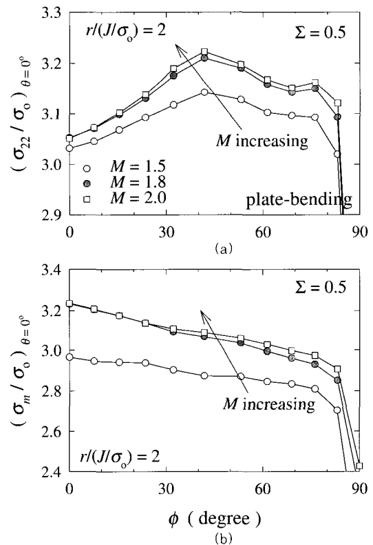
Fig. 10 Normalized (a) crack-tip opening stress, (b) hydrostatic stress along the crack front of plate under remote bending for various M
