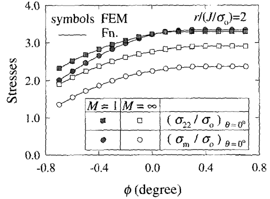
Fig. 13 Effect of T-stress on the hydrostatic stress and the tensile stress at the interface for bimaterials with two extreme plastic strength mismatching: M = 1 and M = \infty
