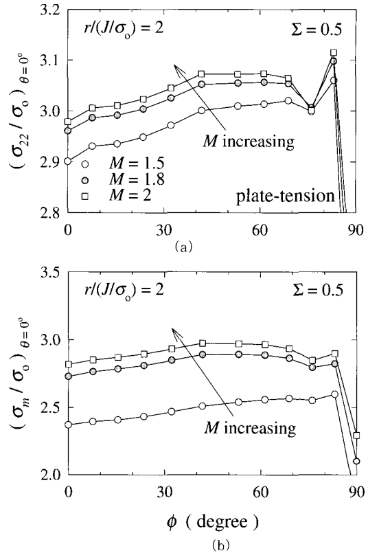
Fig. 7 Normalized stress along the crack front of plate under remote tension for various plastic strength mismatch [(a) crack-tip opening stress, (b) hydrostatic stress]
