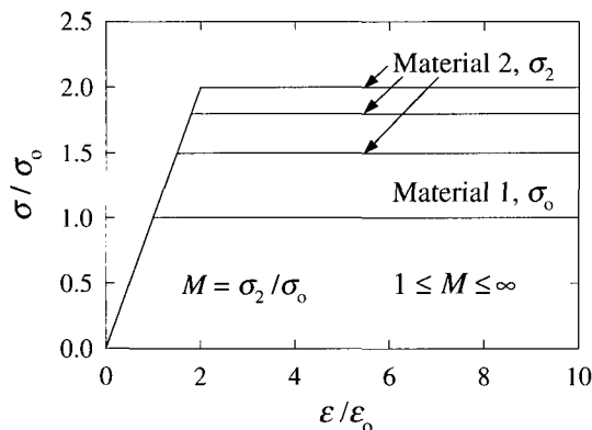
Fig. 5 Material properties of constituents in plastic strength mismatch bimetals
