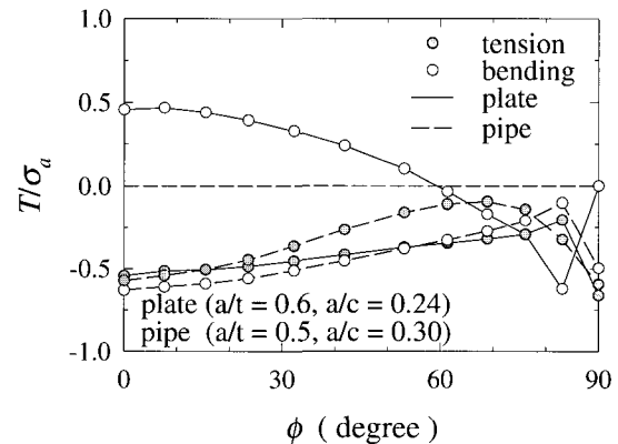
Fig. 4 Normalized T-stress along the crack front of interface-cracked plate and pipe under remote tension and bending
