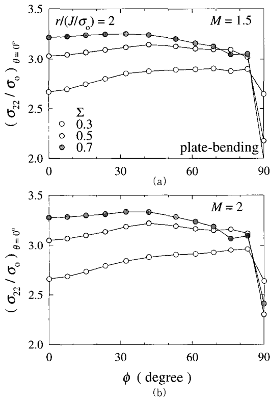
Fig. 9 Normalized crack-tip opening stress along the crack front of plate under remote bending for various load levels [(a) M=1.5 , (b) M=2 ]
