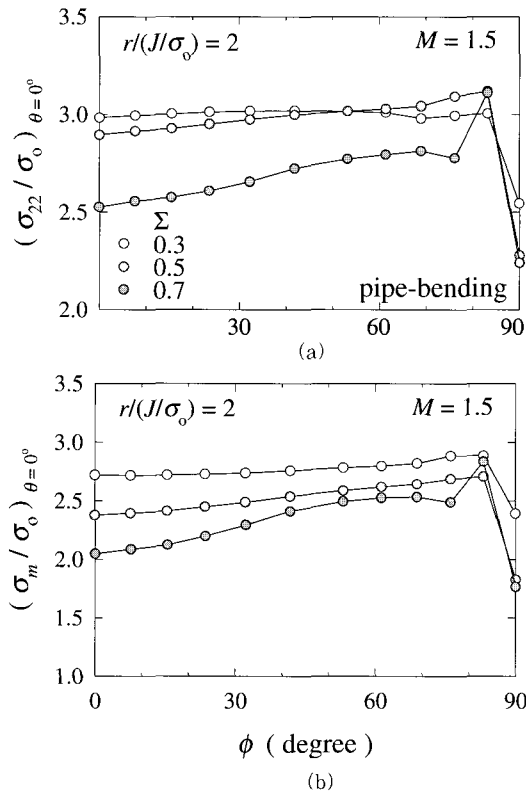
Fig. 11 Normalized (a) crack-tip opening stress and (b) hydrostatic stress along the crack front of pipe under remote bending for various load levels
