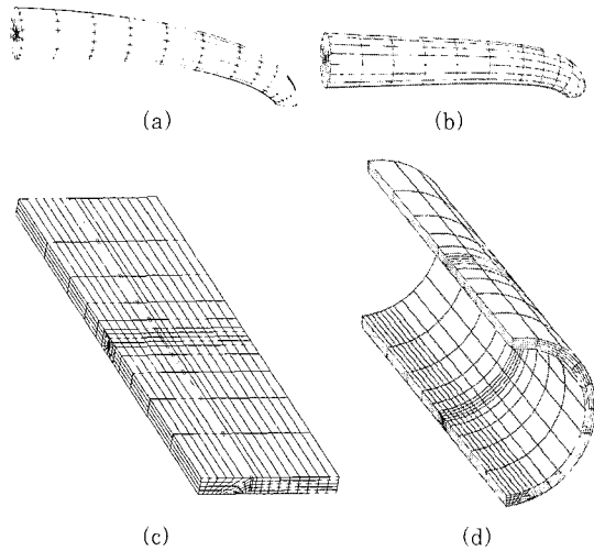
Fig. 2 The 3D mesh near the crack front of (a) plate ( a/t=0.6, a/c=0.24 ), (b) pipe ( a/t=0.5, a/c=0.3 ) and entire 3D mesh of elliptical surface-cracked (c) plate (d) pipe
