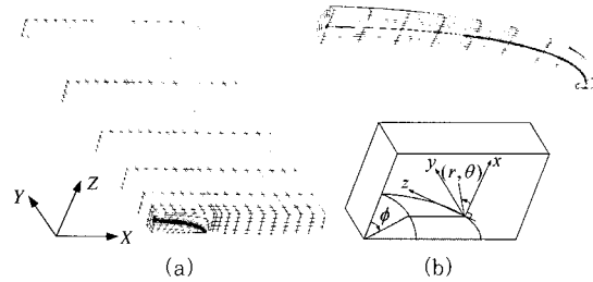
Fig. 3 3D finite element model of the homo-geneous surface cracked plate : (a) the entire 3D mesh and the global coordinate system ( X-Y-Z ) and (b) zoomed 3D mesh for surface crack-front field, and the local coordinate system ( x-y-z )
