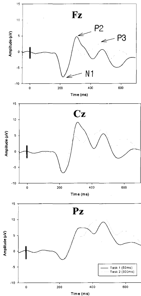
Figure 1. ERP Waveforms from Scalp Midline
