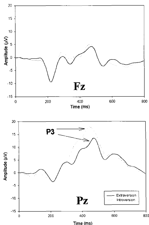
Figure 2. Grand average ERPs at Fz and Pz sites from introversion/extraversion groups for task 1. As shown in figure 12, negative correlation of E and P3 amplitude was higher at parietal area, and lower at frontal area. P3 amplitudes showed the consistent tendency, which introverted subjects' P3 amplitude was higher at parietal sites. Each group was classified according to the extremely polarized E score of NEO-PI-R, and their data were averaged separately ( N=8 for extraversion, and N=9 for introversion). Baseline is omitted and P3 peaks appear with approximately 470 ms latencies.
