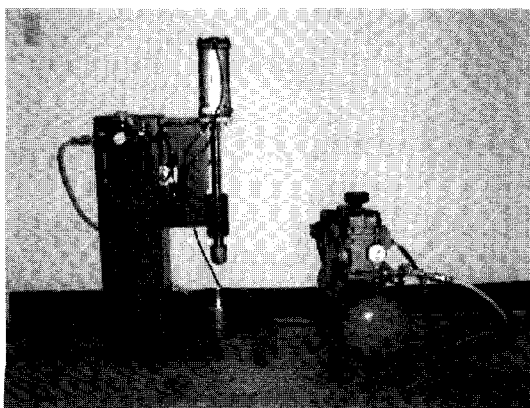
Fig. 1. The impact refining device and a compressor
