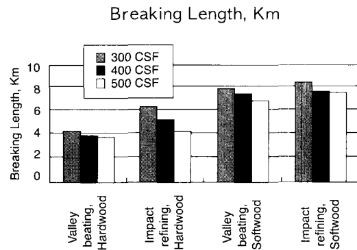
Fig. 5. Differences of breaking lengths caused by different refining methods
