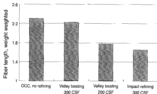
Fig. 14. Fiber length changes by different refining methods
