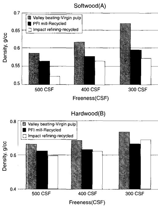
Fig. 10. Density changes after different refining treatments
