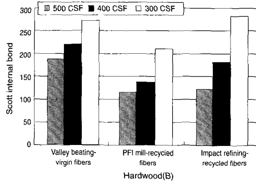
Fig. 13. Scott Internal bonds after different refining treatment A) softwood B) Hardwood
