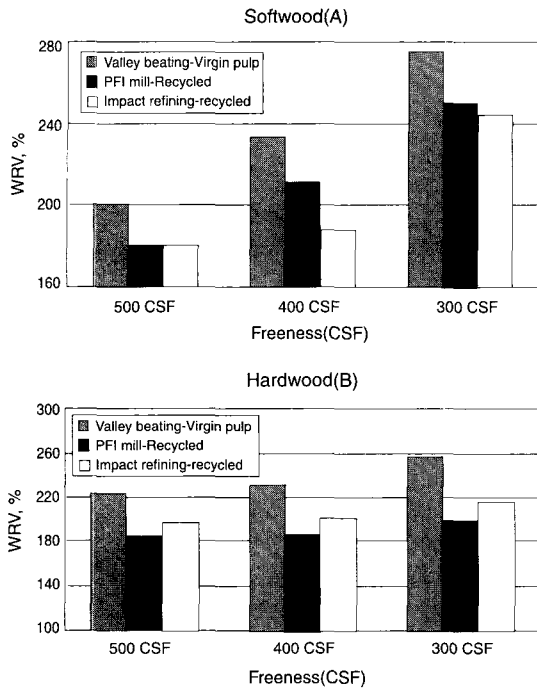
Fig. 9. Water retention values after different refining treatments (A) Softwood, (B) Hardwood
