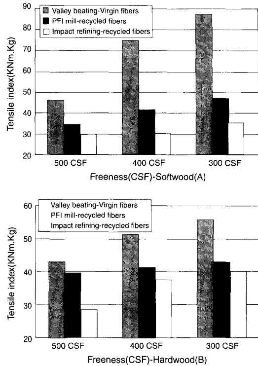
Fig. 11. Tensile indexes after different refining treatments (A) Softwood (B) Hardwood
