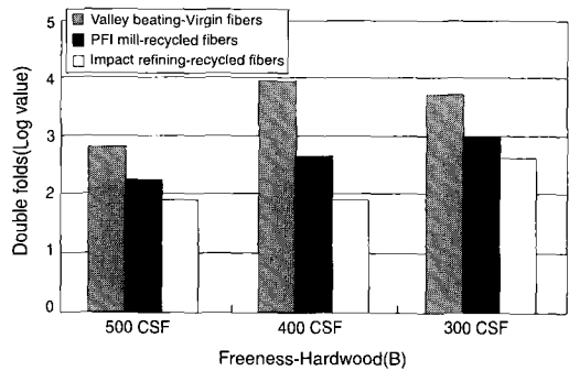
Fig. 12. Folding endurance after different refining treatment A) Softwood B) Hardwood
