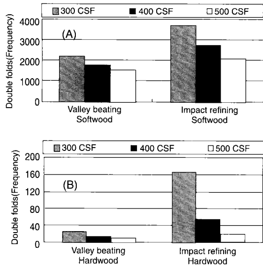
Fig. 6. Differences in folding endurance caused by different refining methods (A) Softwood, (B) Hardwood
