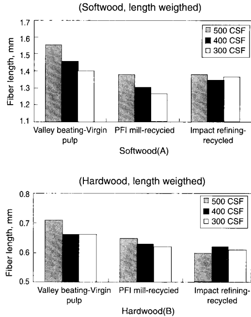
Fig. 8. Fiber length changes after applying different refining methods
