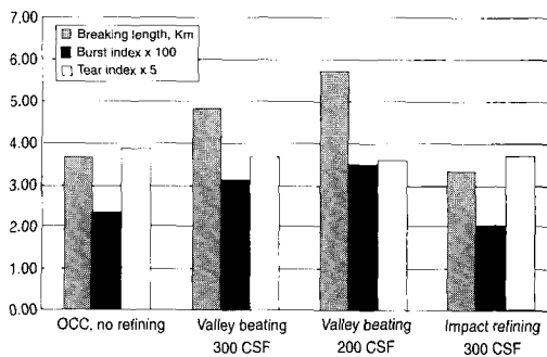
Fig. 15. Comparison of physical property
