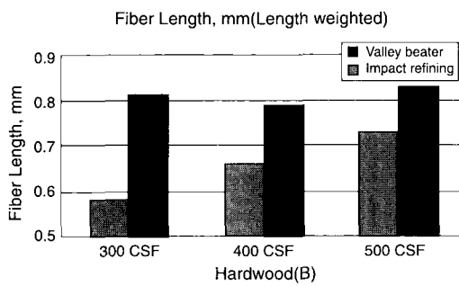
Fig. 2. Fiber length changes by two different refining methods (A) Softwood, (B) Hardwood
