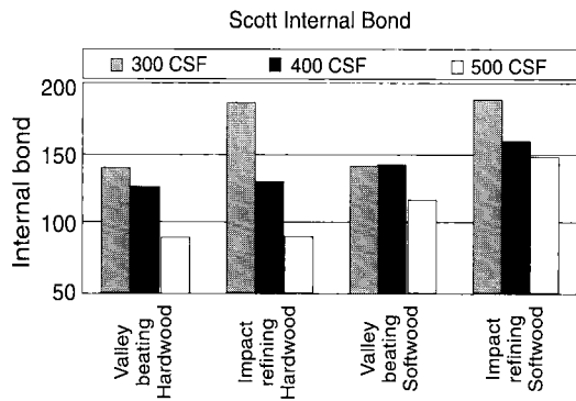
Fig. 7. Differences in Scott internal bond caused by different refining methods
