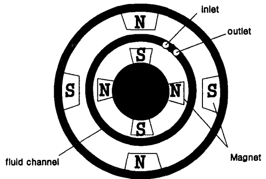
Fig. 1. Cross Sectional Top View of Separator
