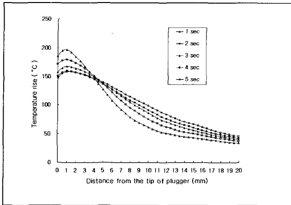
Fig. 7. Temperature changes on the surface of Buchanan pluggers(FM). (setting temperature: 200°C, power level: 10) 0 : Tip of pluggers, 20 : Shank of pluggers
