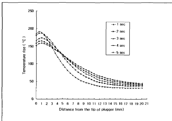
Fig. 9. Temperature changes on the surface of Buchanan pluggers(ML). (setting temperature: 200°C, power level: 10) 0 : Tip of pluggers, 20 : Shank of pluggers
