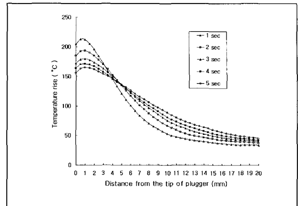
Fig. 8. Temperature changes on the surface of Buchanan pluggers(M). (setting temperature: 200°C, power level: 10) 0 : Tip of pluggers, 20 : Shank of pluggers
