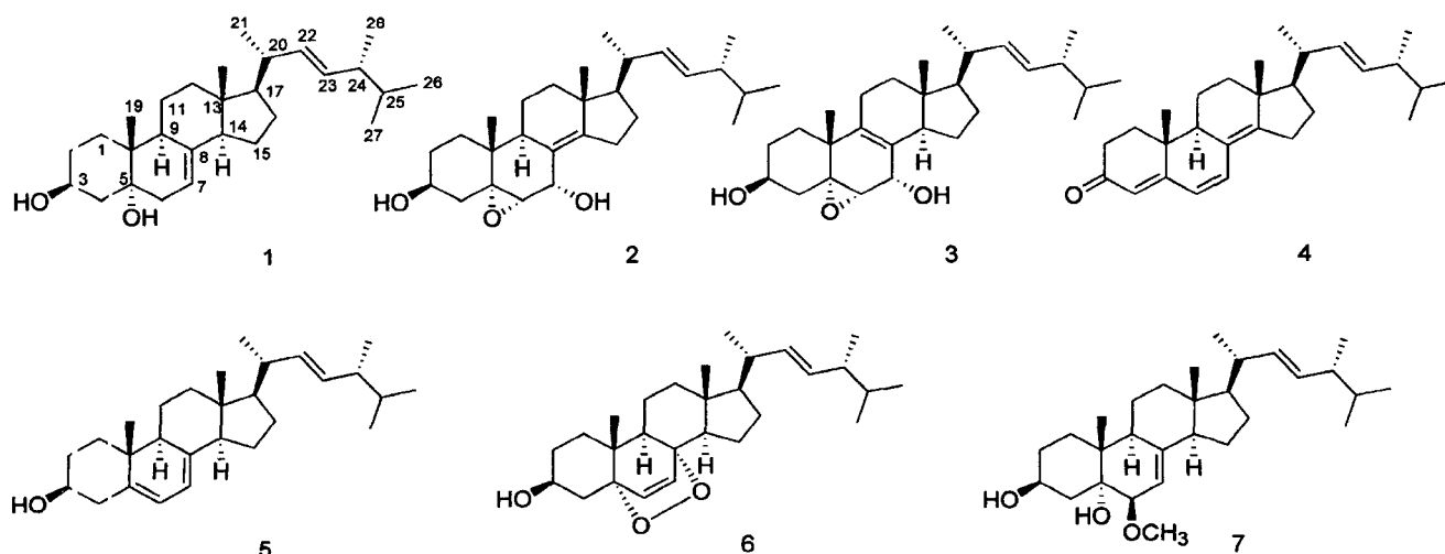
Fig. 1. Structures of compounds 1-7 isolated from Paecilomyces sp. J300.
