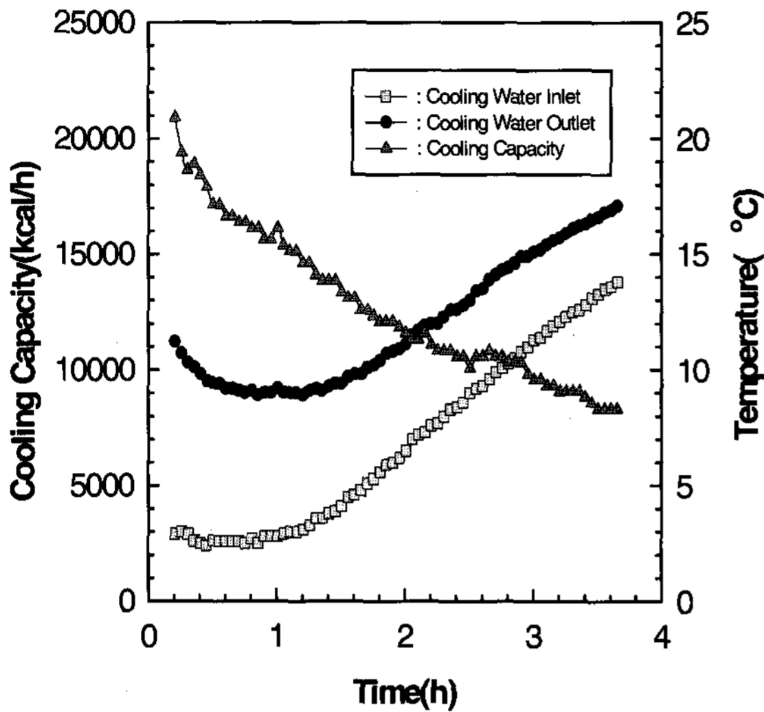
그림 8. Cooling capacity and temperature distribution of inlet and outlet in fan coil unit on discharging process.
