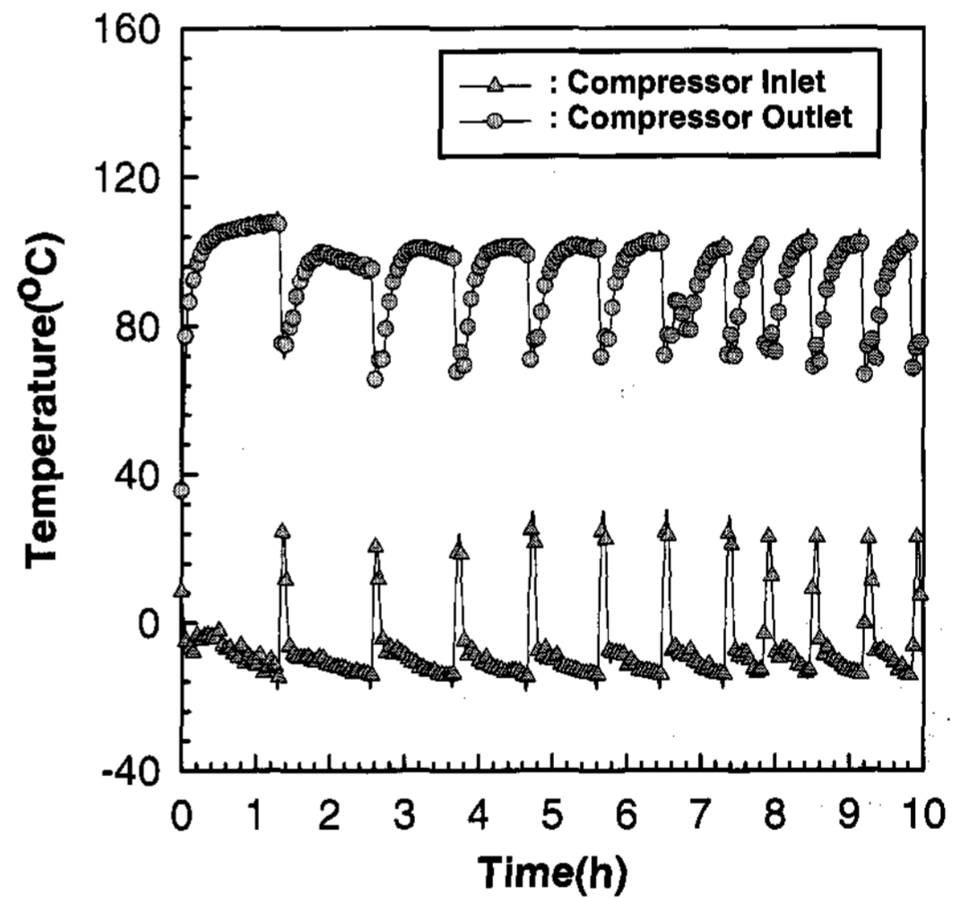
그림 4. Temperature variation at the inlet and outlet of the compressor during the charging process.
