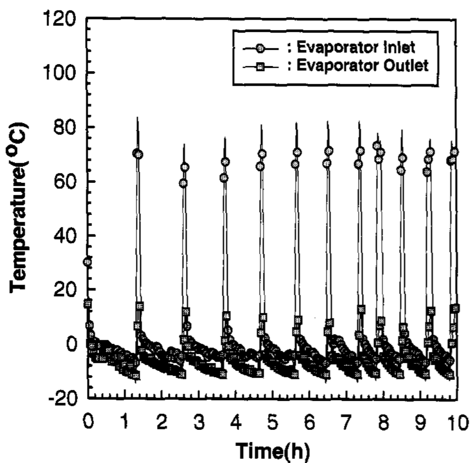
그림 6. Temperature variation at the inlet and outlet of the evaporator during the charging process.
