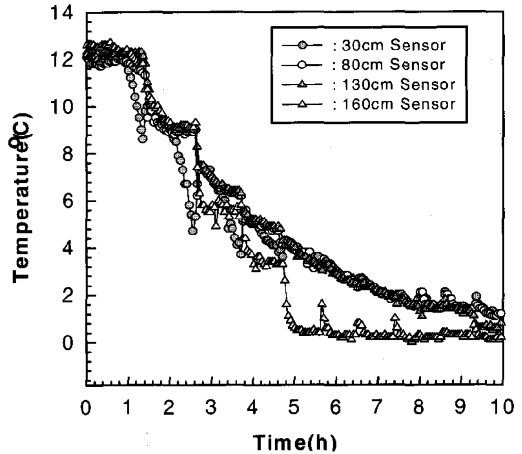
그림 3. Vertical water temperature distribution of in storage tank on charging process.
