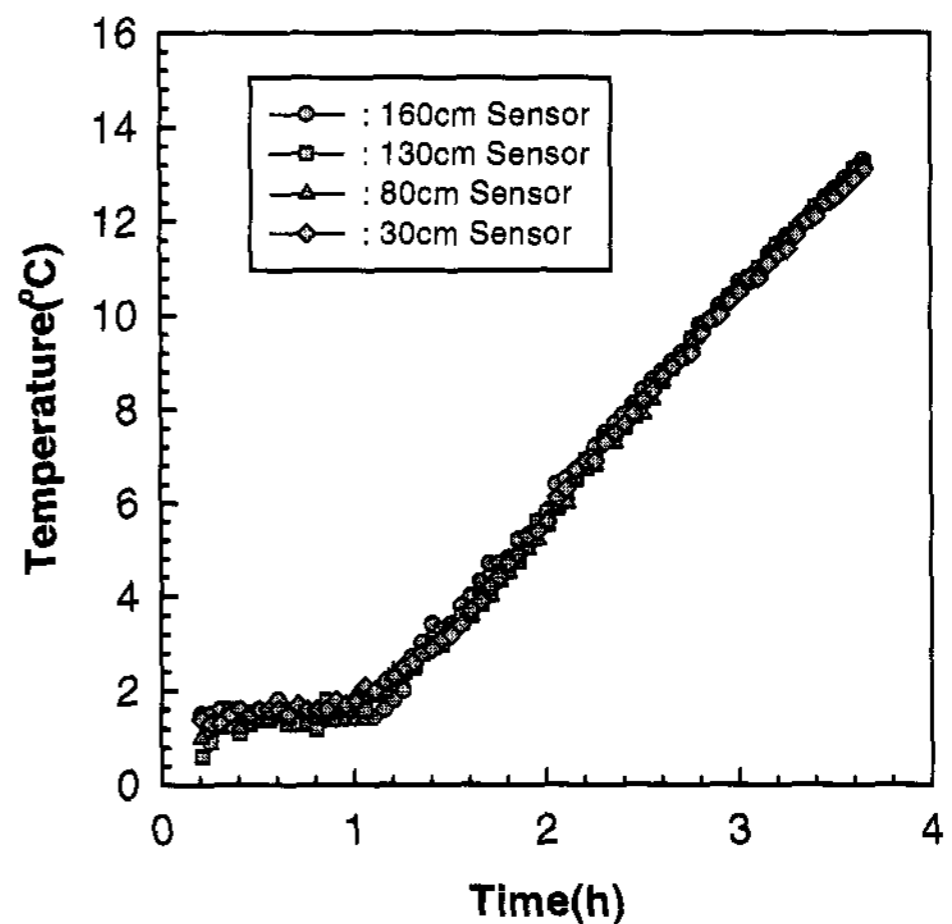
그림 7. Vertical water temperature distribution of in storage tank on discharging process.
