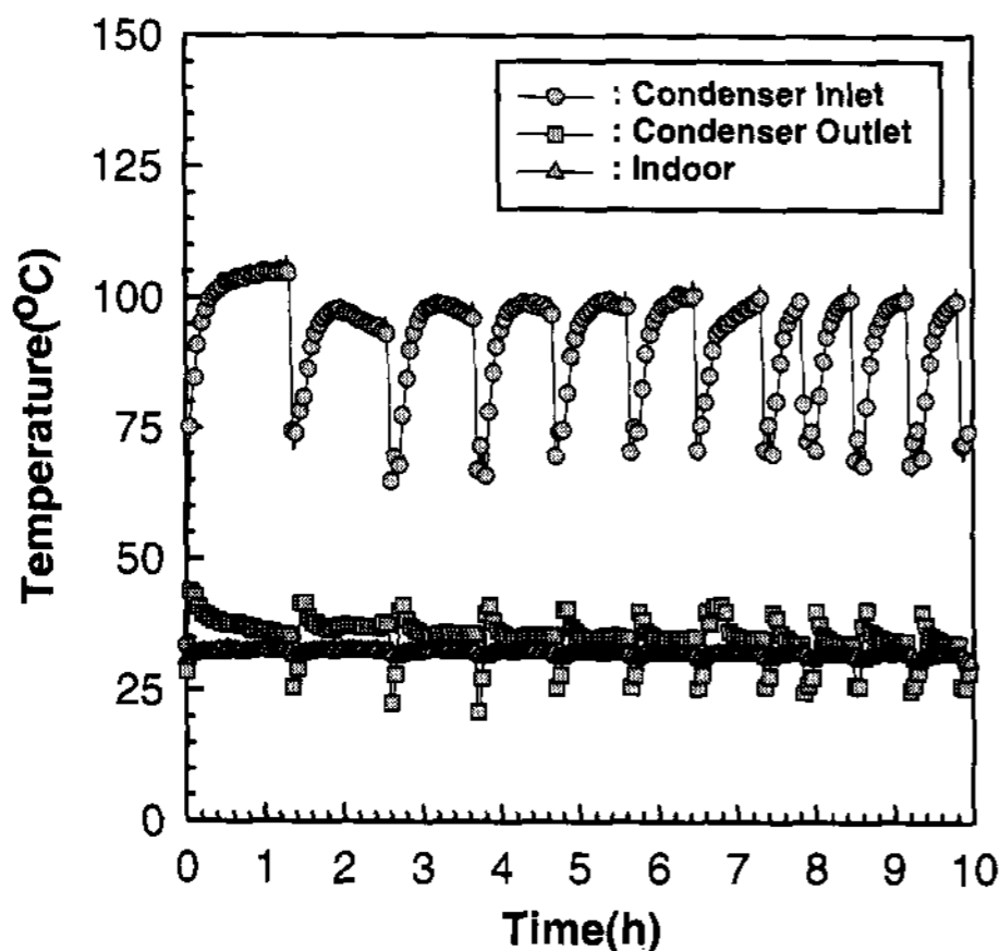
그림 5. Temperature variation at the inlet and outlet of the condenser during the charging process.
