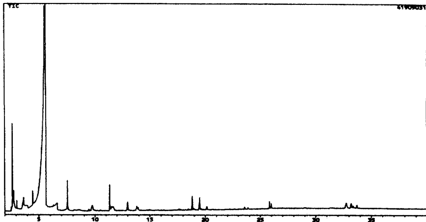
Fig. 1. GC-Mass chromatogrames of refined Joockrhyuk (Bambusae Caulis in Ligua- men)
